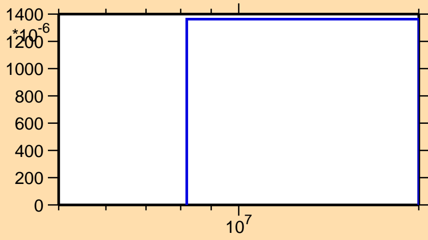
\sigma vs. E for ^{41}\text{Ar}(n,n\alpha)
