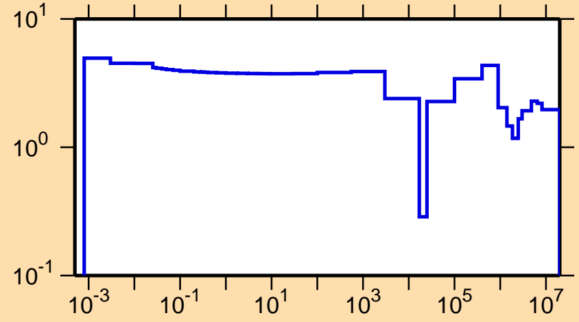
\Delta\sigma/\sigma vs. E for ^{41}\text{Ar}(n,\text{tot.})
