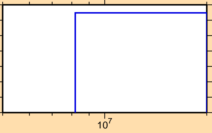
\sigma vs. E for ^{41}\text{Ar}(n,\text{nd})
