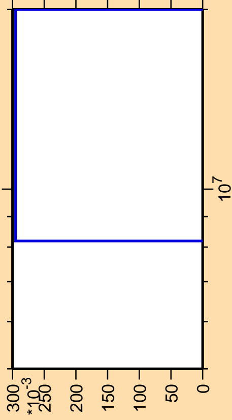
\Delta\sigma/\sigma vs. E for ^{41}\text{Ar}(n,2np)
