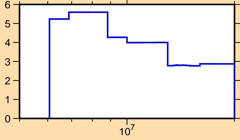
\Delta\sigma/\sigma vs. E for ^{42}\text{Ar}(n,el.)
