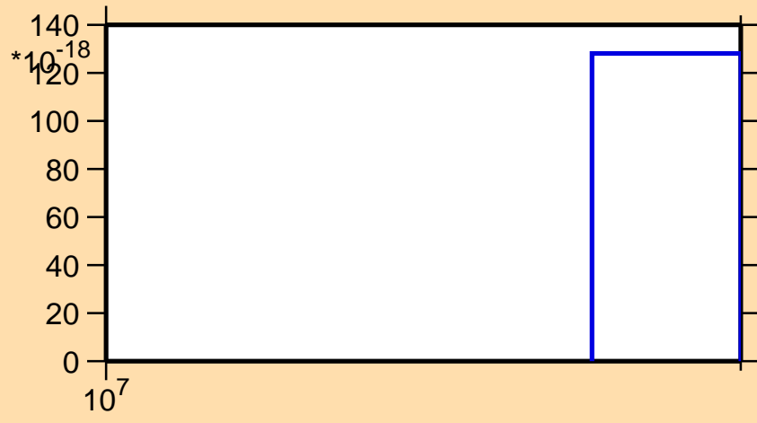
\sigma vs. E for ^{42}\text{Ar}(n,2n\alpha)
