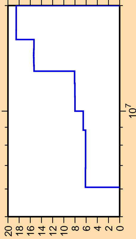
\Delta\sigma/\sigma vs. E for ^{42}\text{Ar}(n,ncont.)
