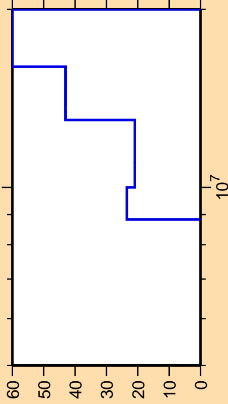
\Delta\sigma/\sigma vs. E for ^{42}\text{Ar}(n,\alpha)
