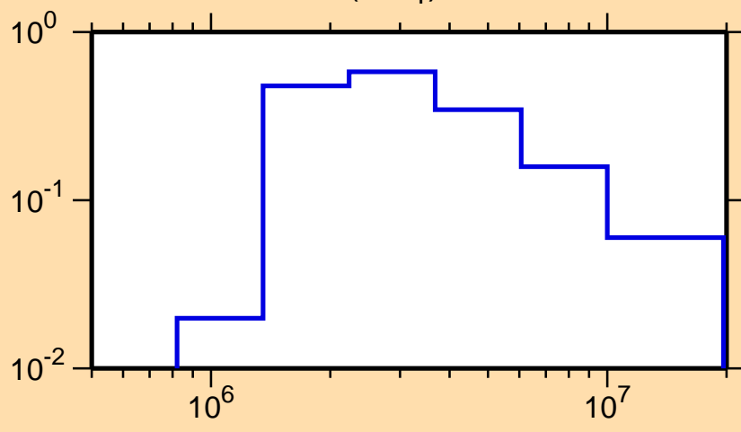
\sigma vs. E for ^{42}\text{Ar}(n,n_1)
