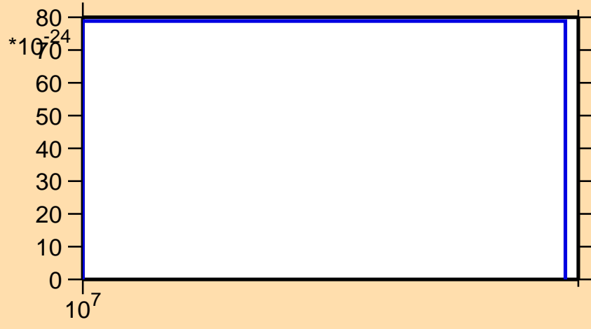
\sigma vs. E for ^{42}\text{Ar}(n,\text{He}3)
