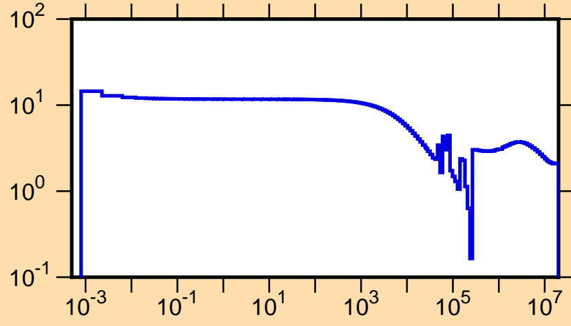
\sigma vs. E for ^{44}\text{Ar}(n,\text{tot.})
