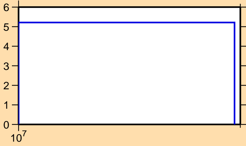
\Delta\sigma/\sigma vs. E for ^{44}\text{Ar}(n,el.)
