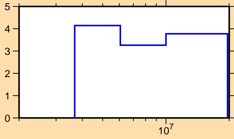
\Delta\sigma/\sigma vs. E for ^{44}\text{Ar}(n,\text{nonel.})
