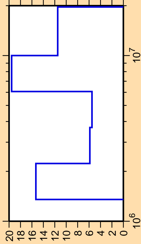
\Delta\sigma/\sigma vs. E for ^{44}\text{Ar}(n,n_4)
