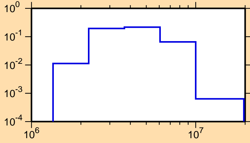
\sigma vs. E for ^{44}\text{Ar}(n,n_4)
