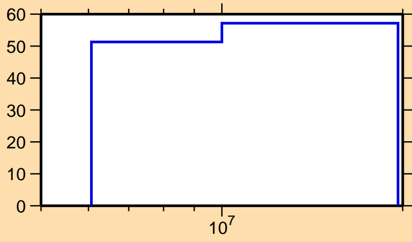
\Delta\sigma/\sigma vs. E for ^{44}\text{Ar}(n,\gamma)
