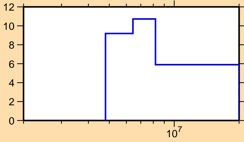
\Delta\sigma/\sigma vs. E for ^{44}\text{Ar}(n,\text{el.})
