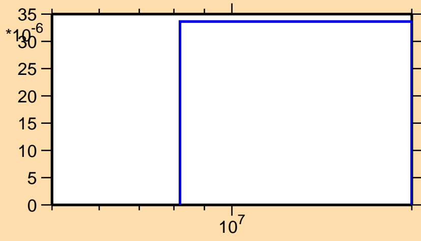
\sigma vs. E for ^{44}\text{Ar}(n,p)
