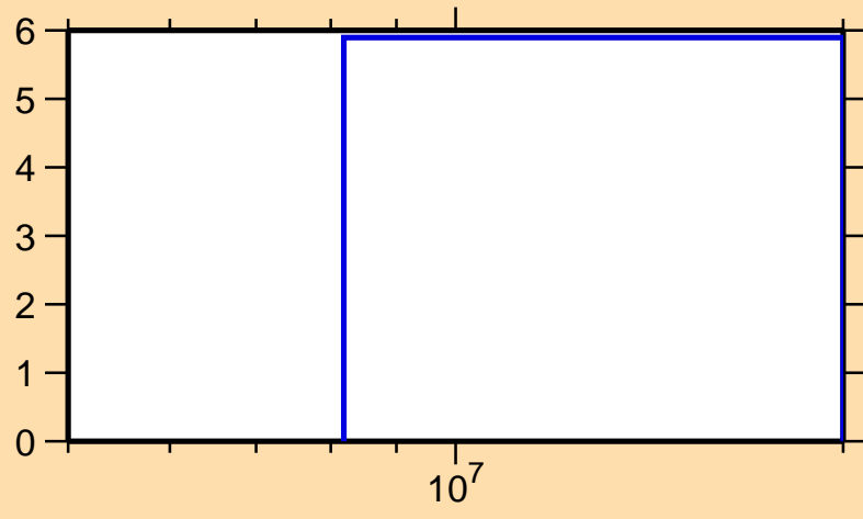
\Delta\sigma/\sigma vs. E for ^{44}\text{Ar}(n,\text{el.})
