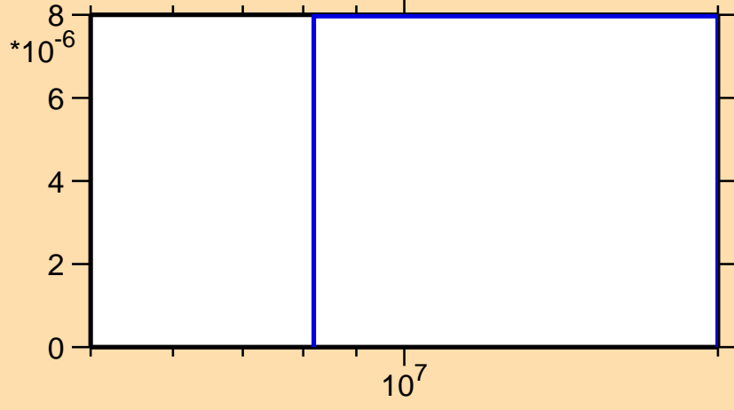
\sigma vs. E for ^{44}\text{Ar}(n,d)
