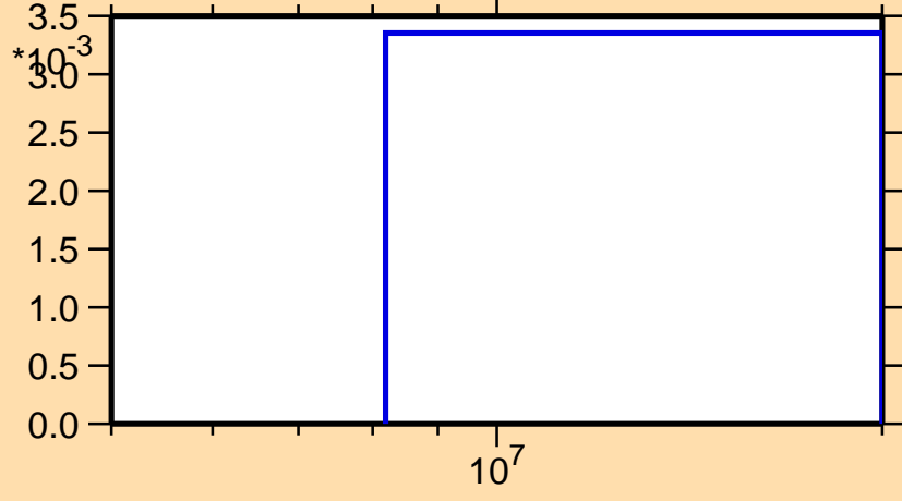
\sigma vs. E for ^{44}\text{Ar}(n,3n)
