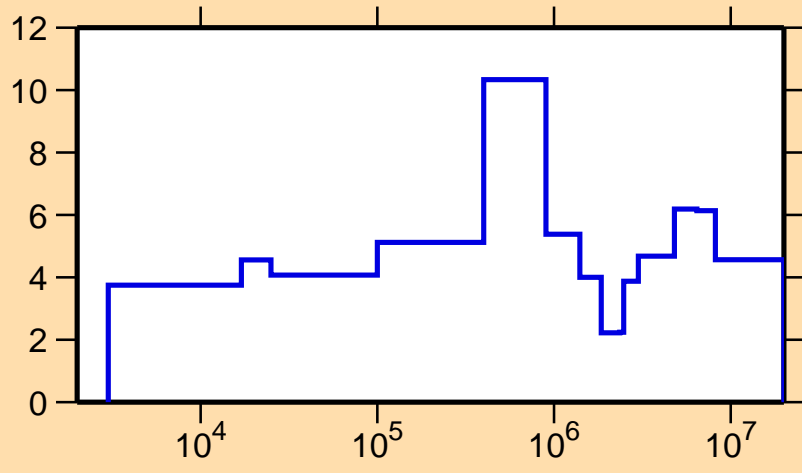
\Delta\sigma/\sigma vs. E for ^{44}\text{Ar}(n,\text{tot.})
