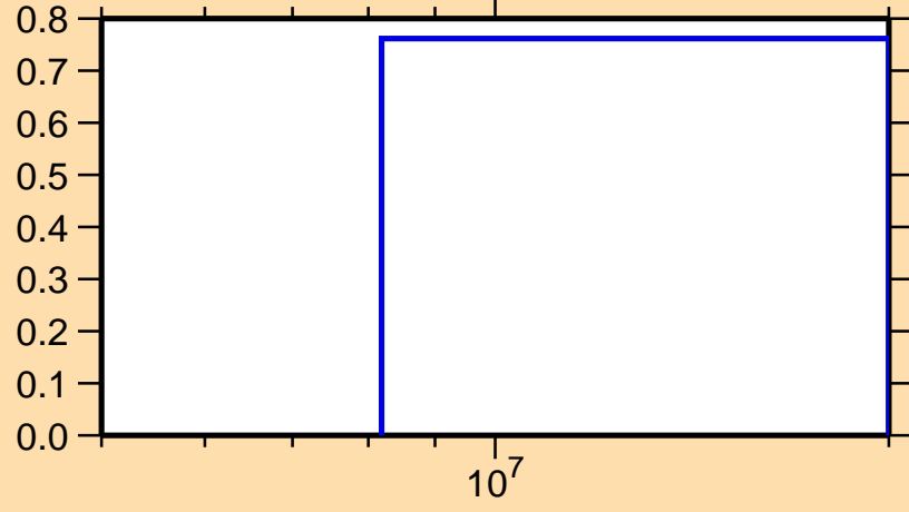
\sigma vs. E for ^{44}\text{Ar}(n,2n)
