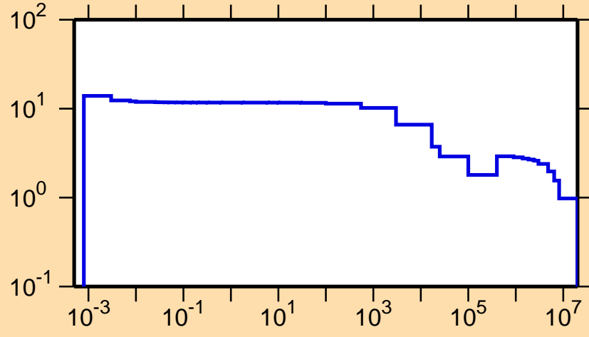
\sigma vs. E for ^{44}\text{Ar}(n,\text{el.})
