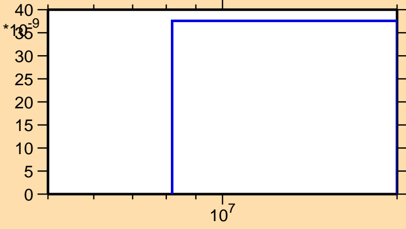
\sigma vs. E for ^{44}\text{Ar}(n,t)
