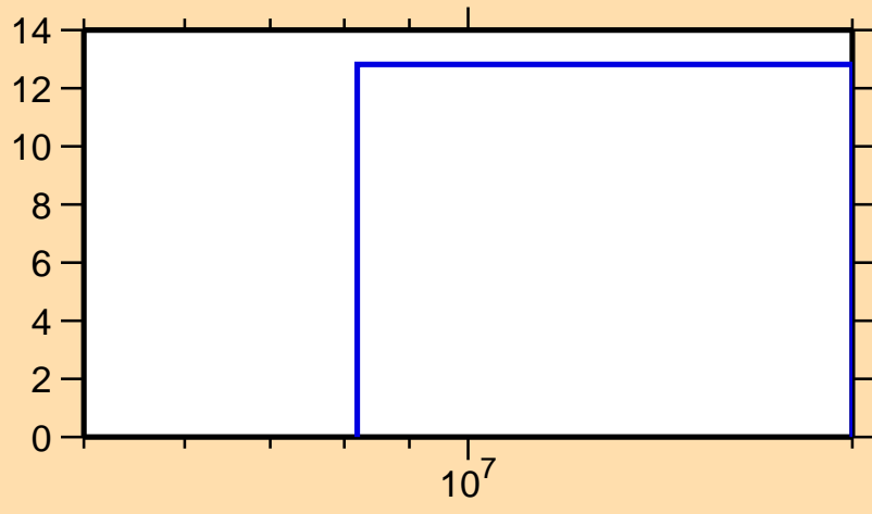
\Delta\sigma/\sigma vs. E for ^{44}\text{Ar}(n,\text{inel.})
