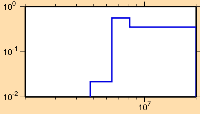
\sigma vs. E for ^{44}\text{Ar}(n,n\text{cont.})
