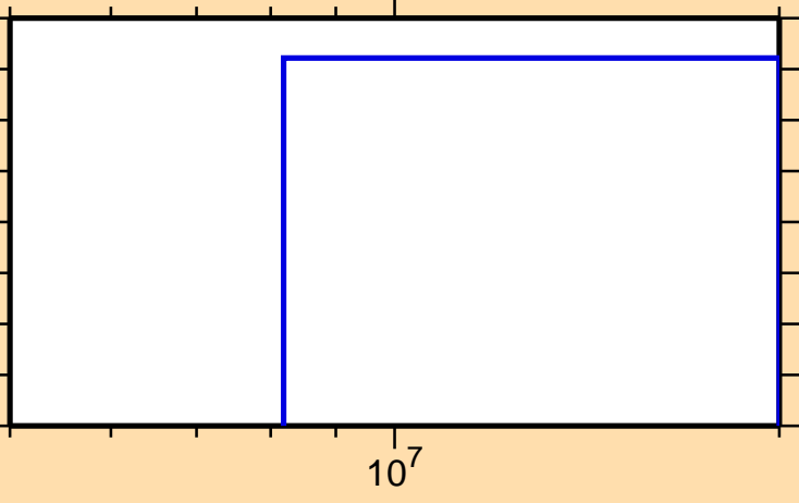
\sigma vs. E for ^{44}\text{Ar}(n,\alpha)
