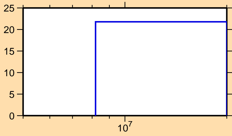
\Delta\sigma/\sigma vs. E for ^{44}\text{Ar}(n,n_1)
