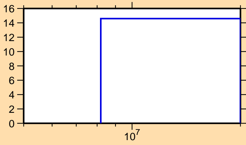
\Delta\sigma/\sigma vs. E for ^{44}\text{Ar}(n,n\text{cont.})
