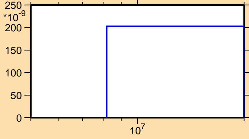
\sigma vs. E for ^{44}\text{Ar}(n,np)
