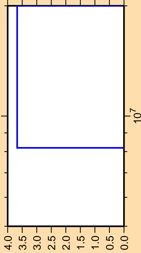
\Delta\sigma/\sigma vs. E for ^{44}\text{Ar}(n,2n)
