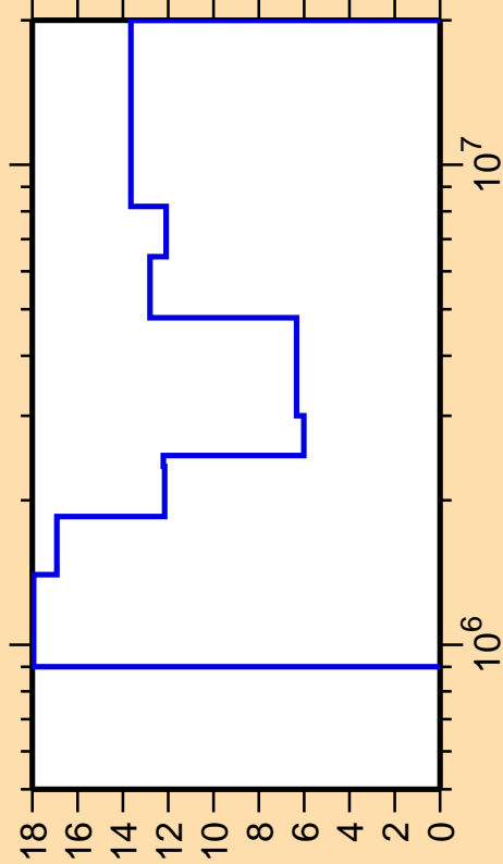
\Delta\sigma/\sigma vs. E for ^{44}\text{Ar}(n,n_2)
