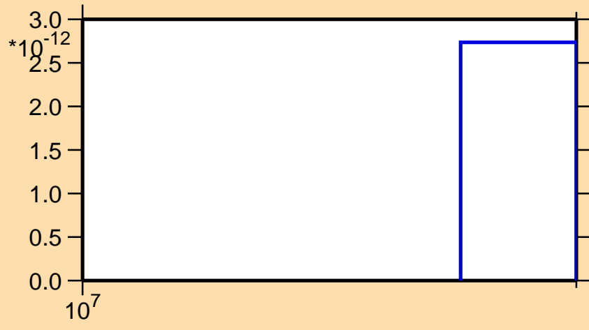
\sigma vs. E for ^{45}\text{Ar}(n,\text{nd})
