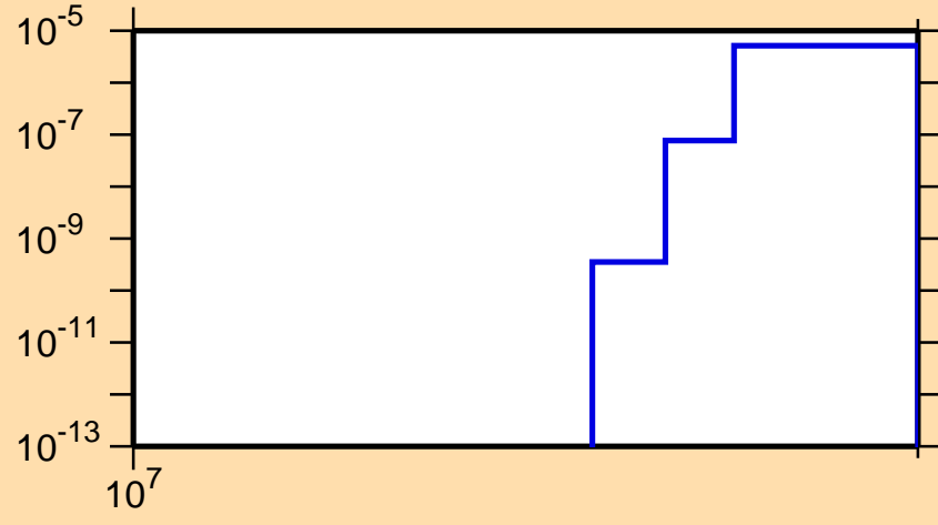
\sigma vs. E for ^{45}\text{Ar}(n,n\alpha)
