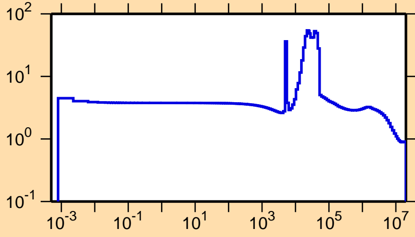
\sigma vs. E for ^{45}\text{Ar}(n,\text{el.})
