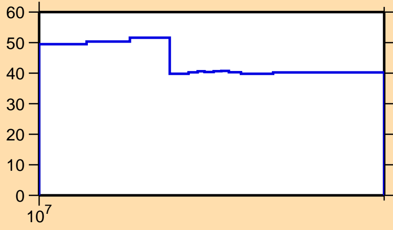
\Delta\sigma/\sigma vs. E for ^{45}\text{Ar}(n,ncont.)
