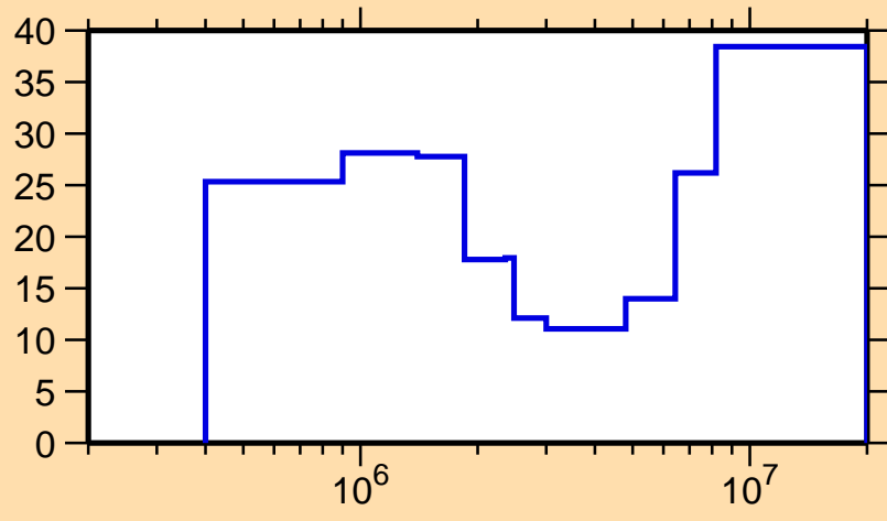
\Delta\sigma/\sigma vs. E for ^{45}\text{Ar}(n,n_1)
