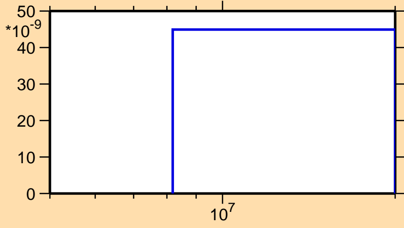
\sigma vs. E for ^{45}\text{Ar}(n,\alpha)
