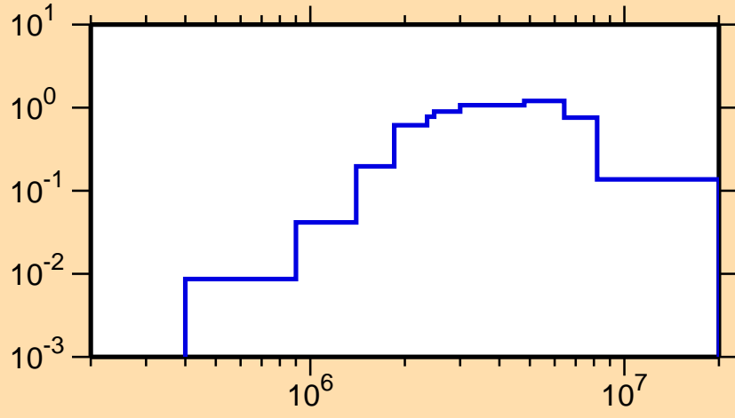
\sigma vs. E for ^{45}\text{Ar}(n,\text{inel.})
