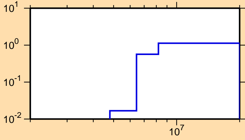
\sigma vs. E for ^{45}\text{Ar}(n,2n)
