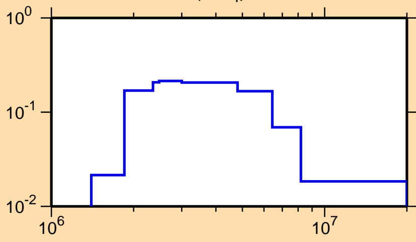
\sigma vs. E for ^{45}\text{Ar}(n,n_4)
