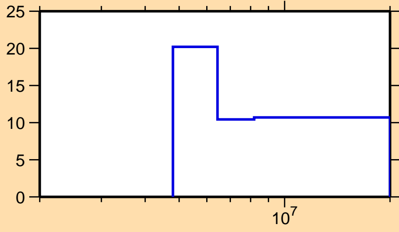
\Delta\sigma/\sigma vs. E for ^{45}\text{Ar}(n,2n)
