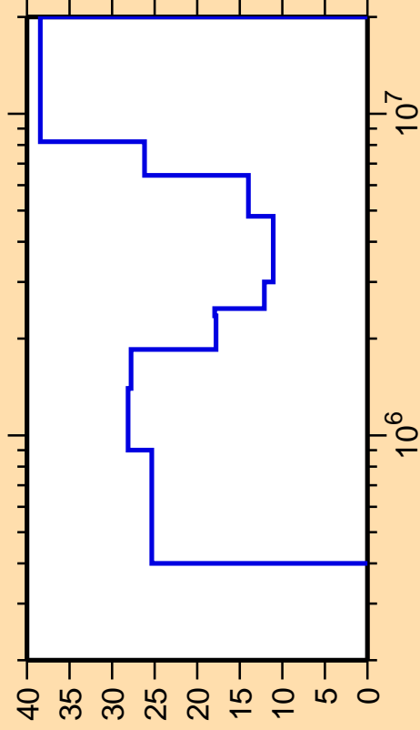
\Delta\sigma/\sigma vs. E for ^{45}\text{Ar}(n,n_1)
