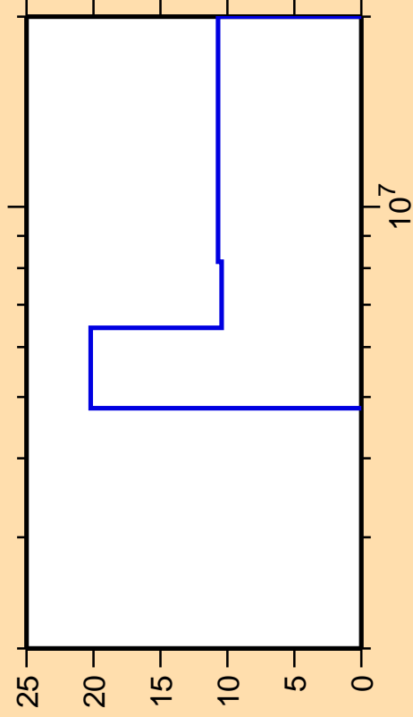
\Delta\sigma/\sigma vs. E for ^{45}\text{Ar}(n,2n)
