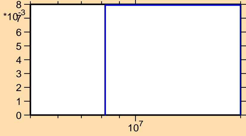
\sigma vs. E for ^{45}\text{Ar}(n,3n)
