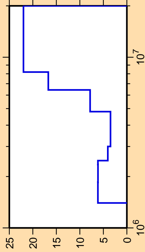
\Delta\sigma/\sigma vs. E for ^{45}\text{Ar}(n,n_3)
