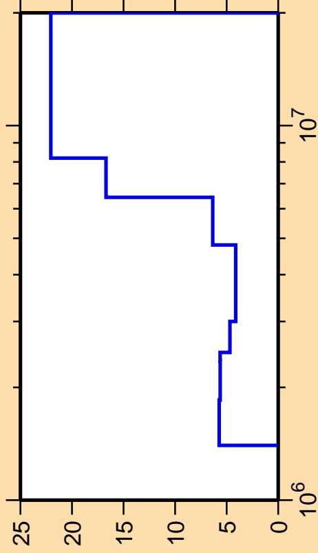
\Delta\sigma/\sigma vs. E for ^{45}\text{Ar}(n,n_4)
