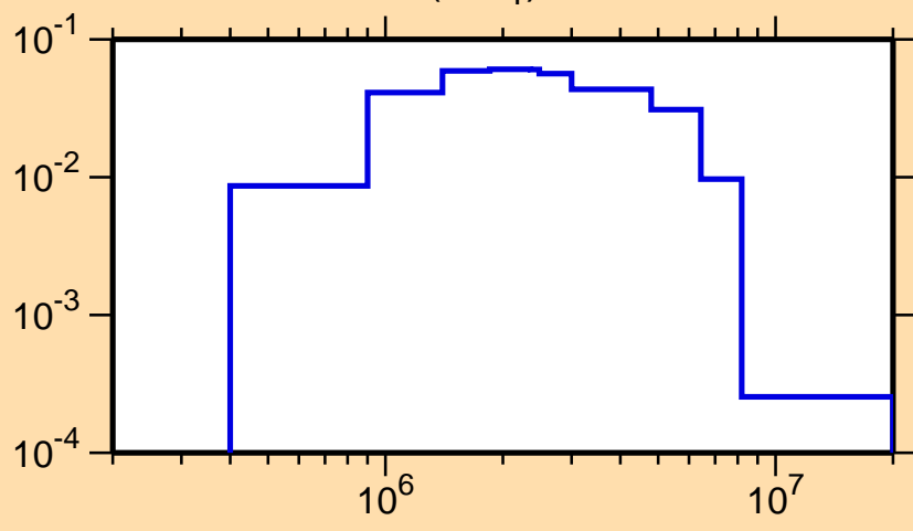
\sigma vs. E for ^{45}\text{Ar}(n,n_1)
