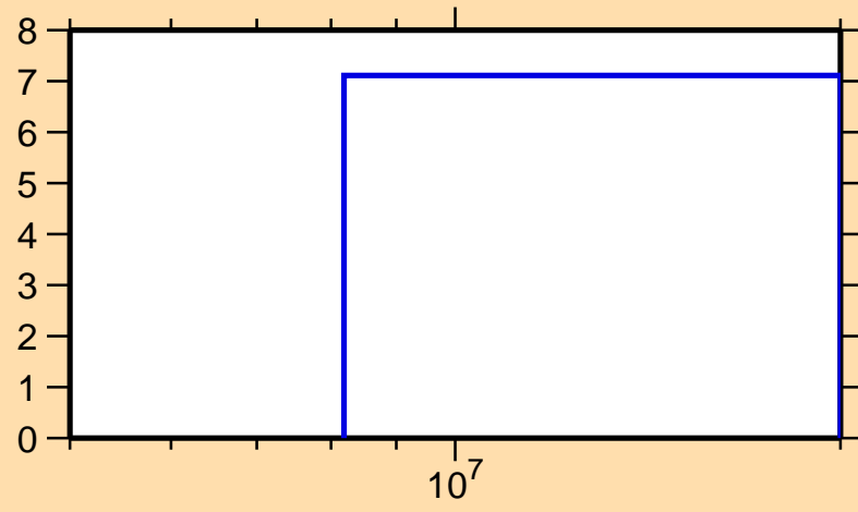
\Delta\sigma/\sigma vs. E for ^{45}\text{Ar}(n,el.)
