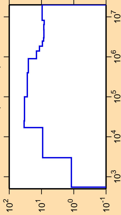
\Delta\sigma/\sigma vs. E for ^{45}\text{Ar}(n,\text{nonel.})
