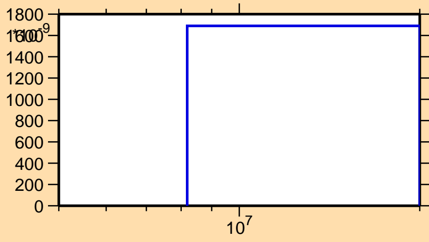
\sigma vs. E for ^{45}\text{Ar}(n,t)
