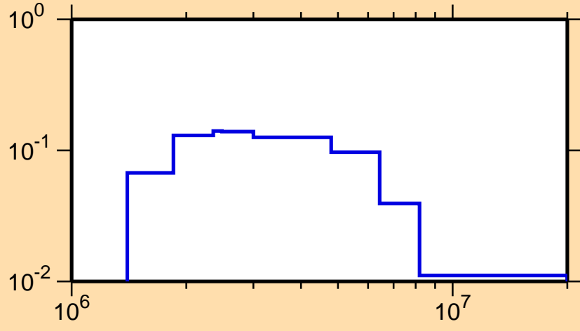
\sigma vs. E for ^{45}\text{Ar}(n,n_3)
