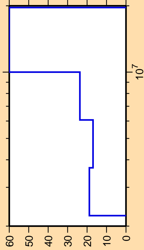
\Delta\sigma/\sigma vs. E for ^{46}\text{Ar}(n,n_4)
