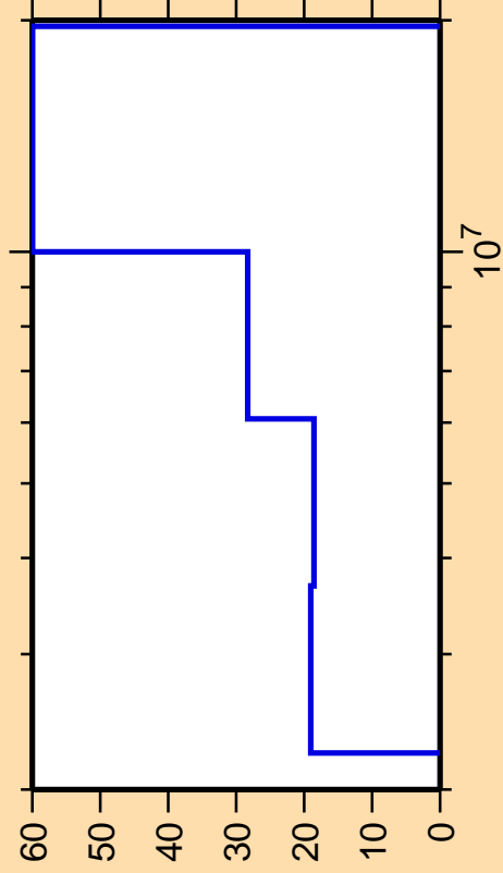
\Delta\sigma/\sigma vs. E for ^{46}\text{Ar}(n,n_3)
