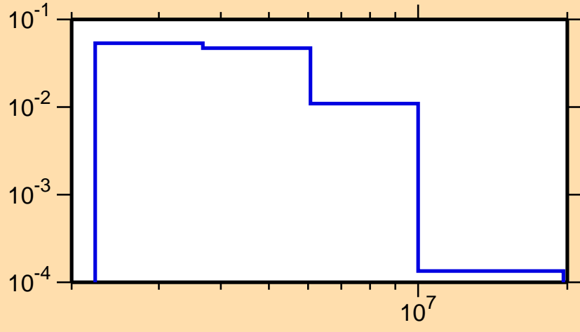
\sigma vs. E for ^{46}\text{Ar}(n,n_3)
