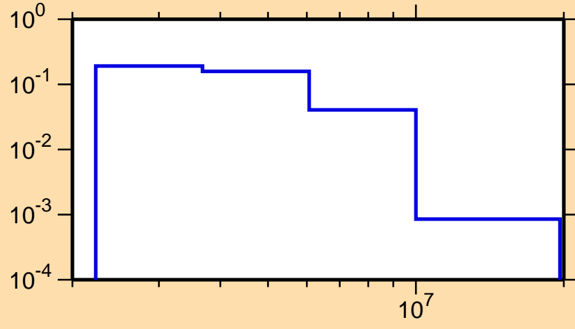
\sigma vs. E for ^{46}\text{Ar}(n,n_2)
