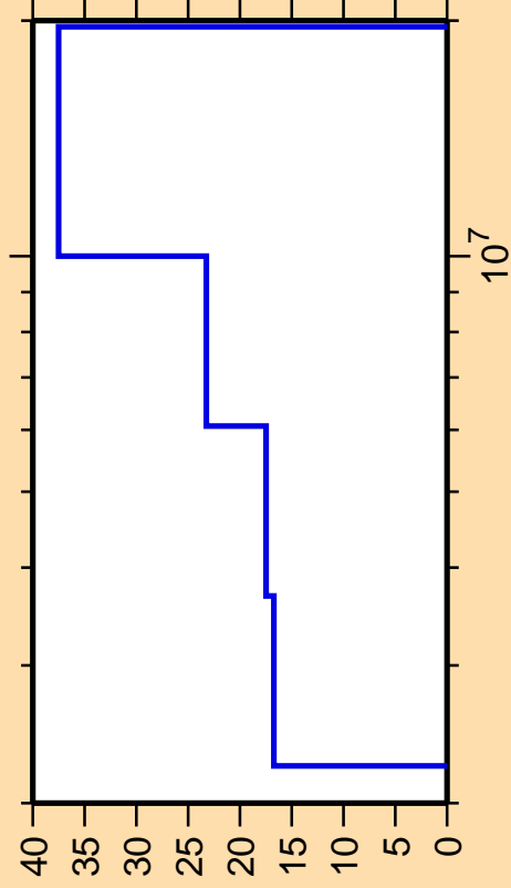
\Delta\sigma/\sigma vs. E for ^{46}\text{Ar}(n,n_2)
