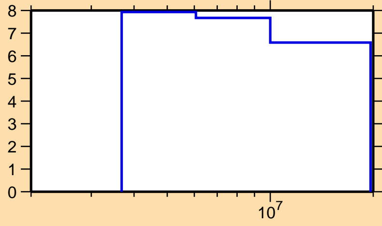
\Delta\sigma/\sigma vs. E for ^{46}\text{Ar}(n,tot.)
