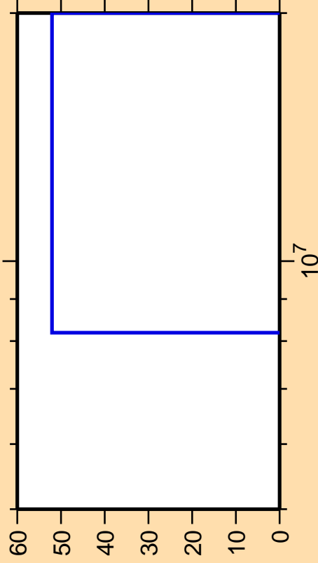
\Delta\sigma/\sigma vs. E for ^{46}\text{Ar}(n,\gamma)
