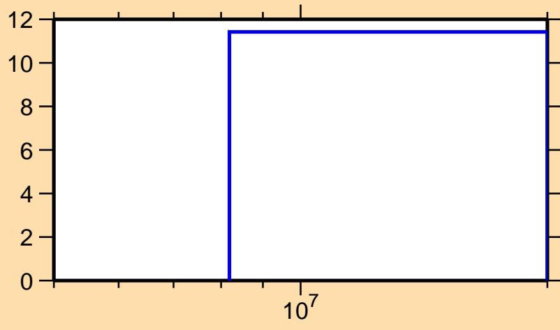
\Delta\sigma/\sigma vs. E for ^{46}\text{Ar}(n,el.)
