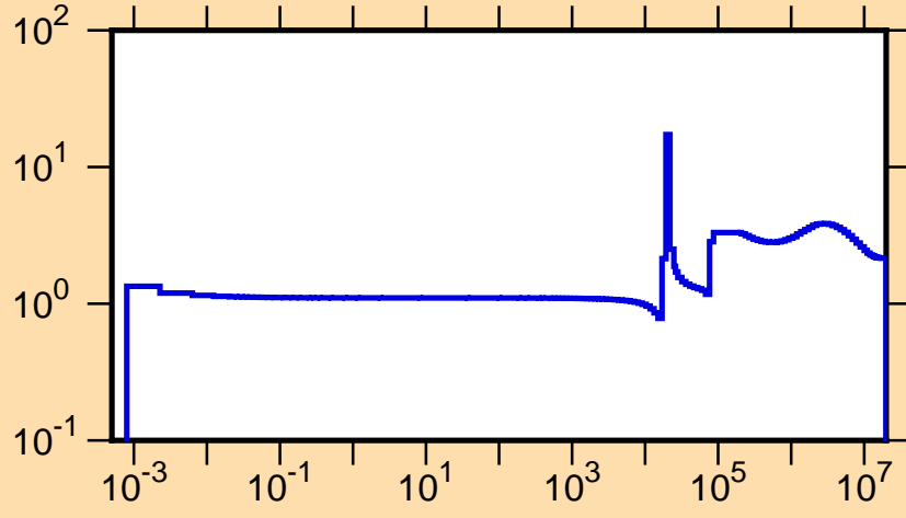
\sigma vs. E for ^{47}\text{Ar}(n,\text{tot.})
