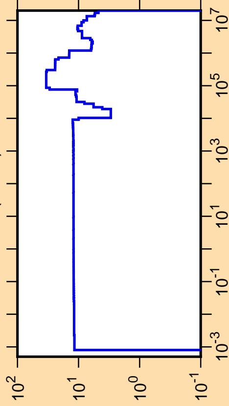
\Delta\sigma/\sigma vs. E for ^{47}\text{Ar}(n,\text{tot.})
