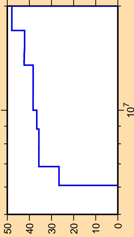
\Delta\sigma/\sigma vs. E for ^{47}\text{Ar}(n,\gamma)
