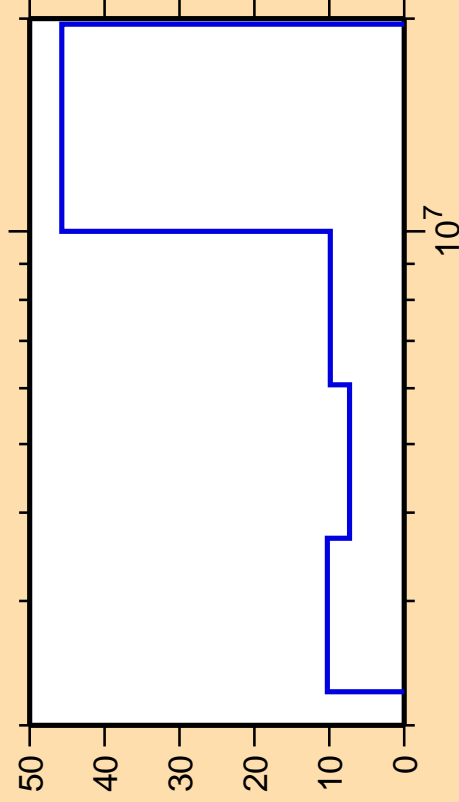
\Delta\sigma/\sigma vs. E for ^{47}\text{Ar}(n,n_3)
