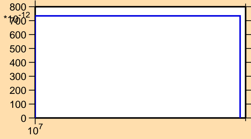
\sigma vs. E for ^{47}\text{Ar}(n,d)
