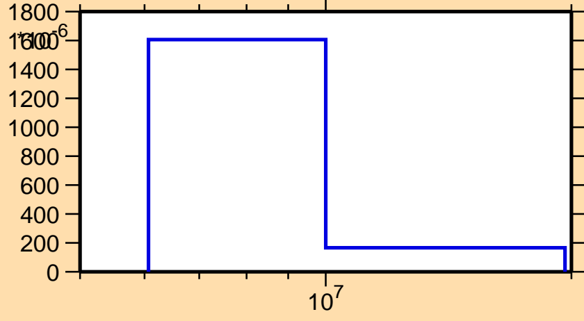
\sigma vs. E for ^{47}\text{Ar}(n,n\text{cont.})
