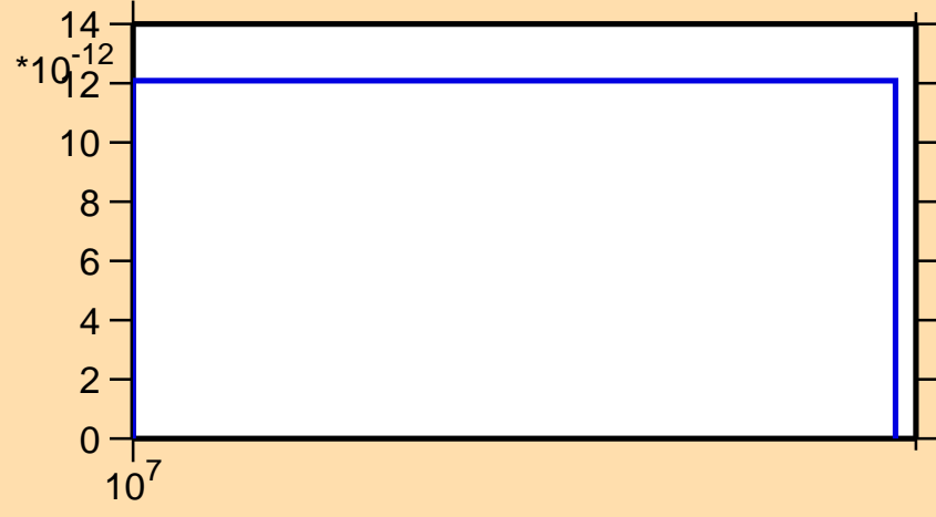
\sigma vs. E for ^{47}\text{Ar}(n,n\alpha)
