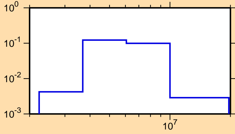
\sigma vs. E for ^{47}\text{Ar}(n,n_4)
