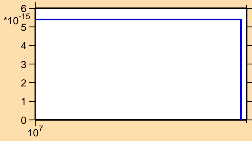
\sigma vs. E for ^{47}\text{Ar}(n,np)
