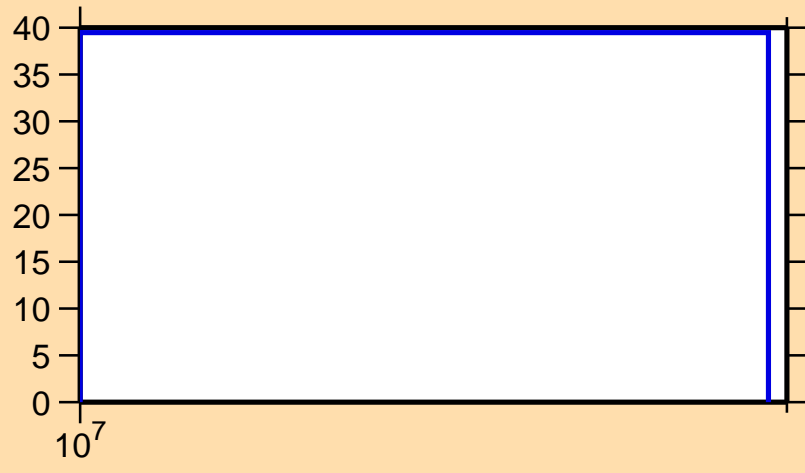
\Delta\sigma/\sigma vs. E for ^{47}\text{Ar}(n,p)
