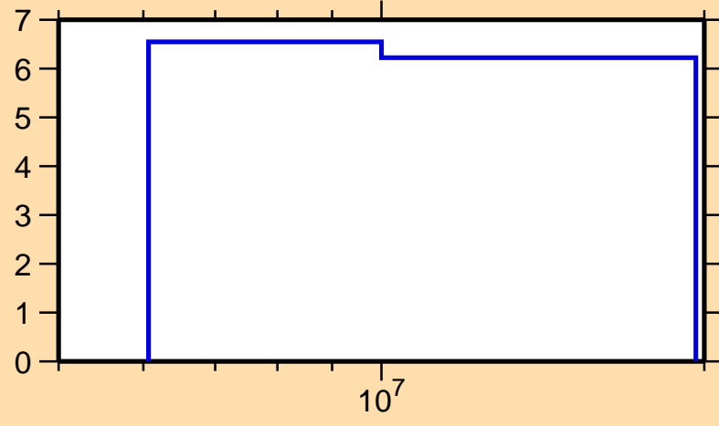
\Delta\sigma/\sigma vs. E for ^{47}\text{Ar}(n,\text{nonel.})
