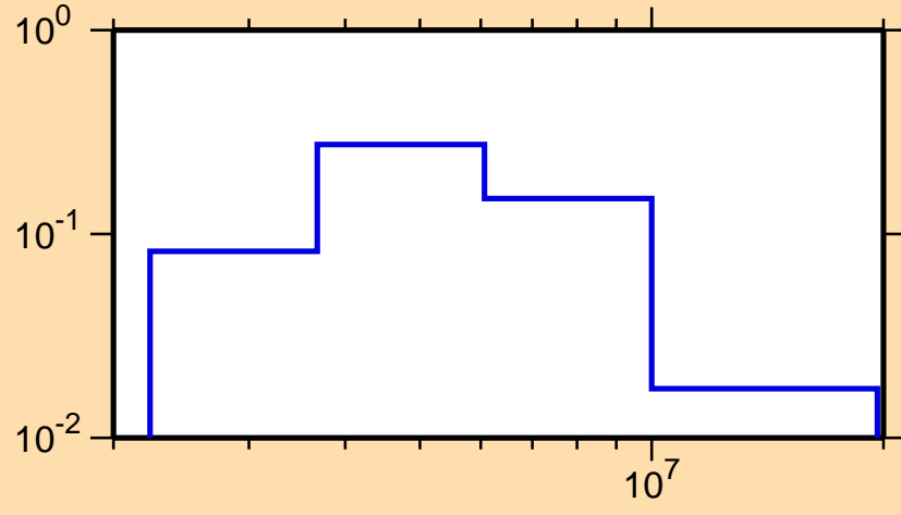
\sigma vs. E for ^{47}\text{Ar}(n,n_3)
