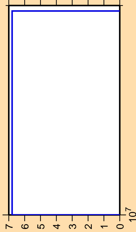
\Delta\sigma/\sigma vs. E for ^{47}\text{Ar}(n,np)
