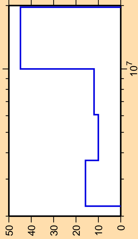
\Delta\sigma/\sigma vs. E for ^{47}\text{Ar}(n,n_4)
