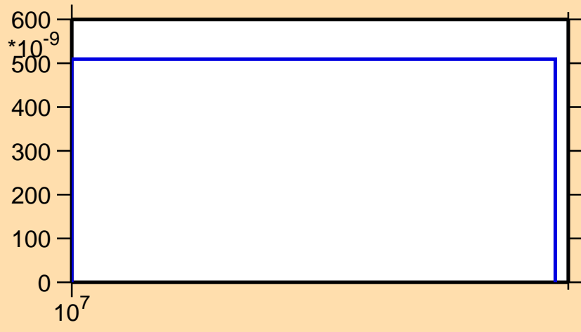
\sigma vs. E for ^{47}\text{Ar}(n,p)
