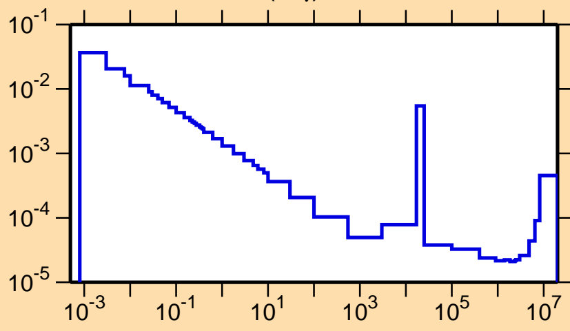
\sigma vs. E for ^{47}\text{Ar}(n,\gamma)
