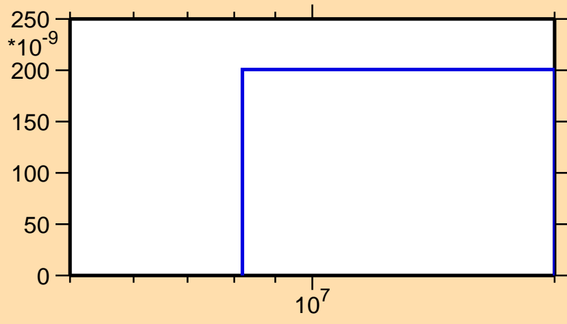
\sigma vs. E for ^{67}\text{As}(n,\text{pt})
