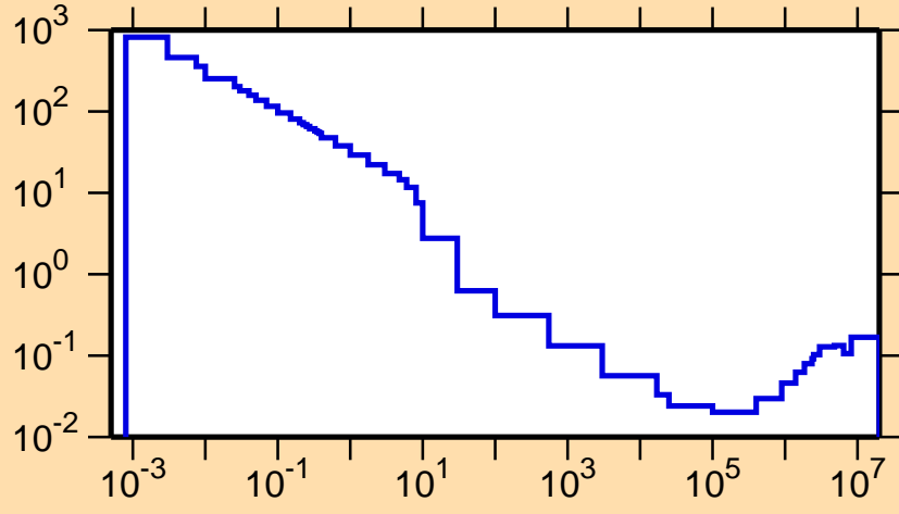
\sigma vs. E for ^{67}\text{As}(n,\alpha)
