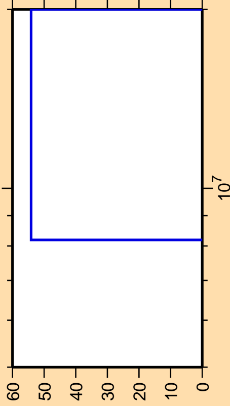
\Delta\sigma/\sigma vs. E for ^{67}\text{As} (mt 45)
