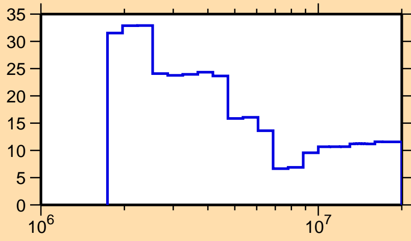
\Delta\sigma/\sigma vs. E for ^{69}\text{As}(n,n_1)
