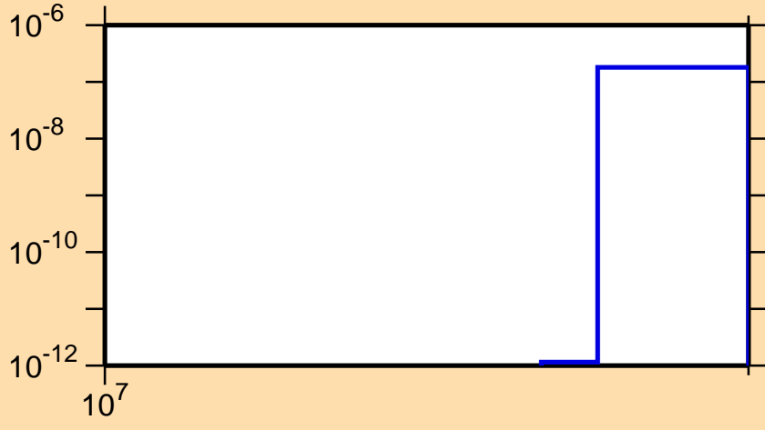
\sigma vs. E for ^{69}\text{As}(n,pt)
