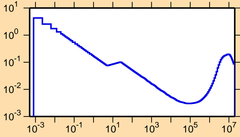
\sigma vs. E for ^{69}\text{As}(n,\alpha)
