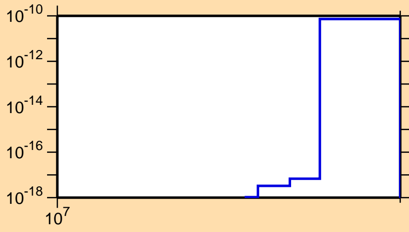
\sigma vs. E for ^{69}\text{As} (mt 34)
