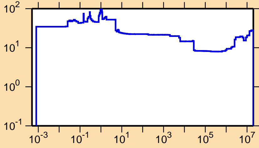
\Delta\sigma/\sigma vs. E for ^{69}\text{As}(n,p)
