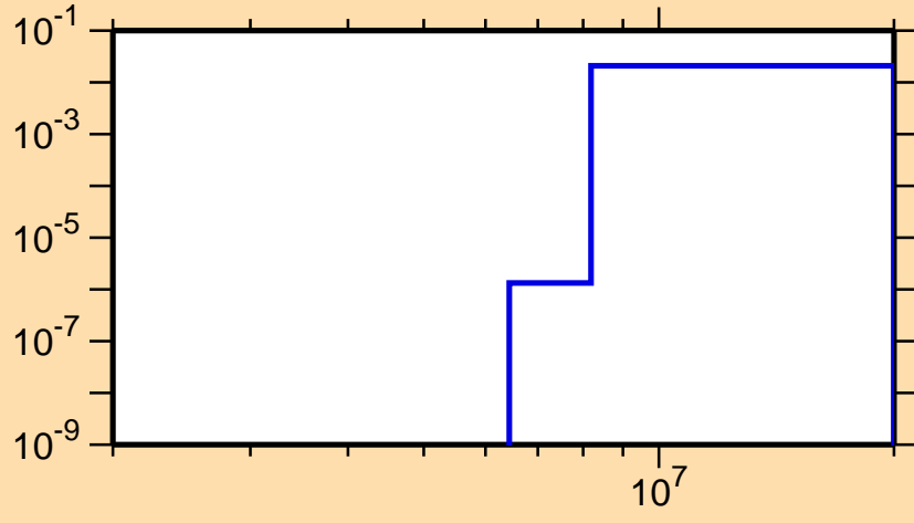
\sigma vs. E for ^{69}\text{As}(n,n\alpha)
