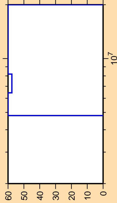
\Delta\sigma/\sigma vs. E for ^{69}\text{As}(n,n\alpha)
