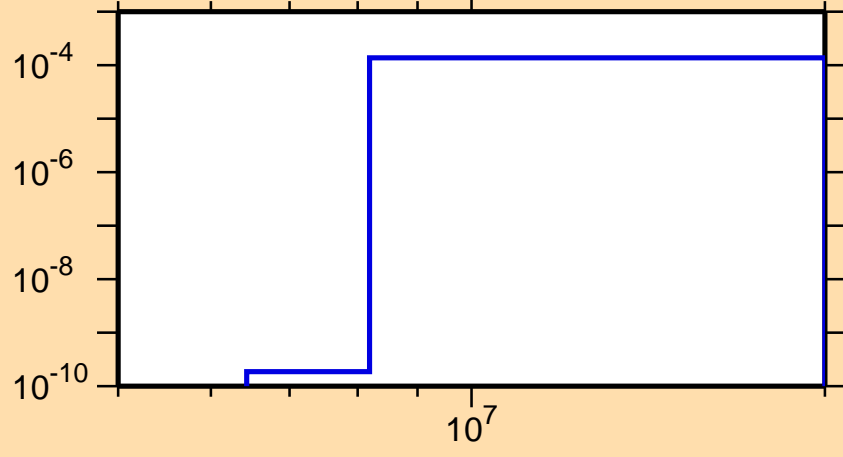
\sigma vs. E for ^{69}\text{As}(n,\text{He3})
