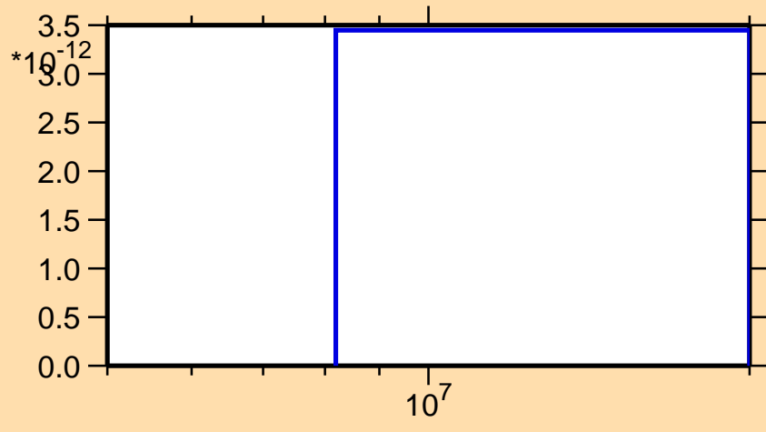
\sigma vs. E for ^{69}\text{As}(n,nt)
