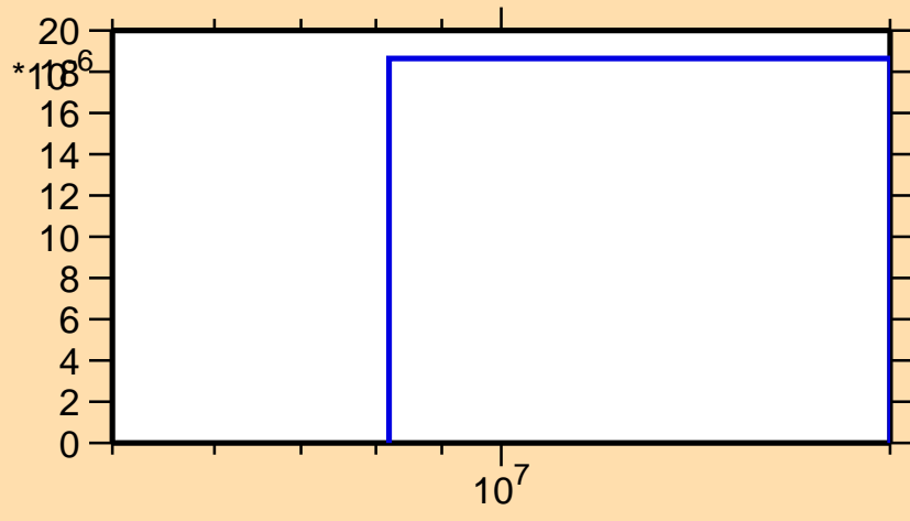
\sigma vs. E for ^{69}\text{As} (mt 45)
