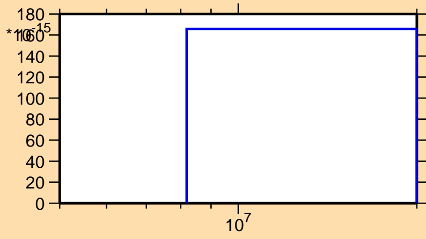
\sigma vs. E for ^{69}\text{As}(n,2n\alpha)
