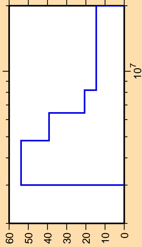
\Delta\sigma/\sigma vs. E for ^{69}\text{As}(n,np)
