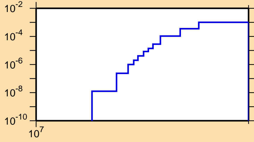
\sigma vs. E for ^{70}\text{As}(n,nd)
