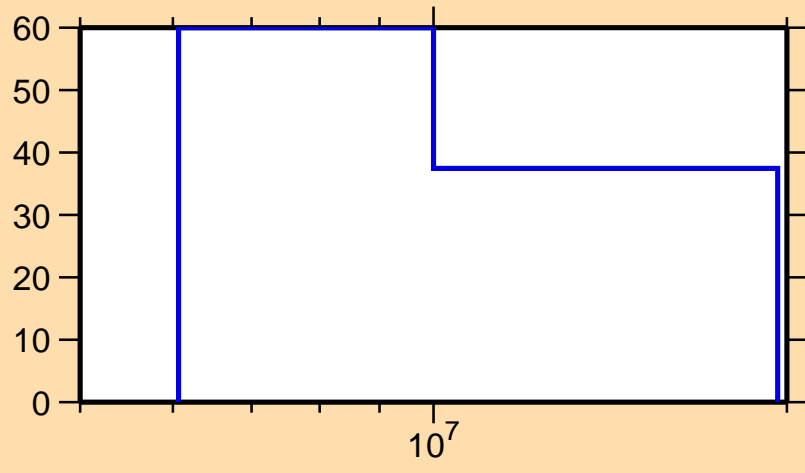
\Delta\sigma/\sigma vs. E for ^{70}\text{As}(n,2n)
