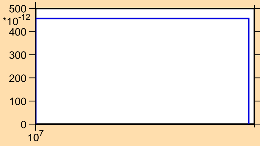
\sigma vs. E for ^{70}\text{As} (mt 34)
