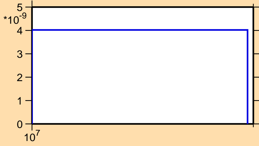
\sigma vs. E for ^{70}\text{As}(n,2n\alpha)
