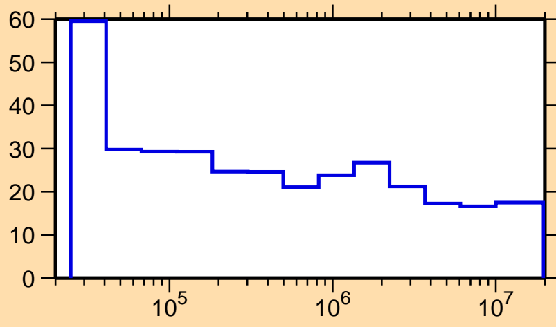
\Delta\sigma/\sigma vs. E for ^{70}\text{As}(n,\text{inel.})
