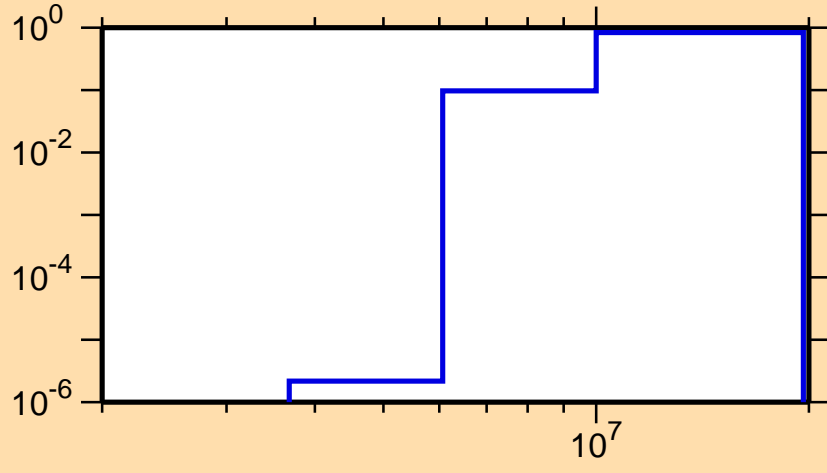
\sigma vs. E for ^{70}\text{As}(n,np)
