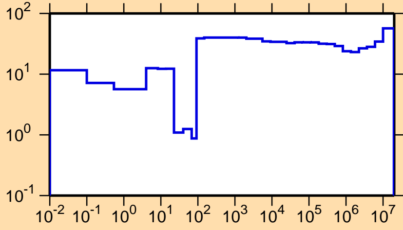
\Delta\sigma/\sigma vs. E for ^{70}\text{As}(n,\gamma)
