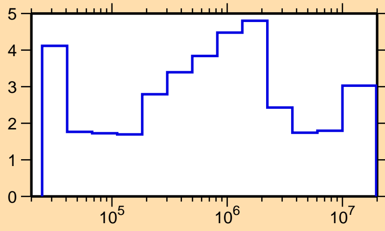
\Delta\sigma/\sigma vs. E for ^{70}\text{As}(n,\text{tot.})
