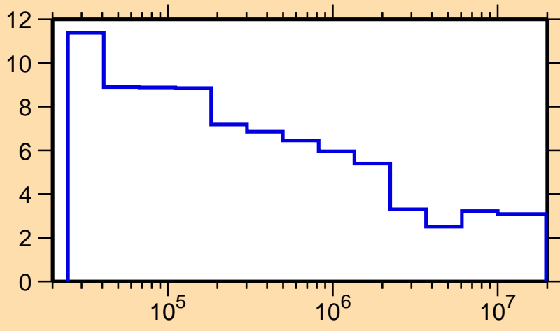
\Delta\sigma/\sigma vs. E for ^{70}\text{As}(n,\text{nonel.})
