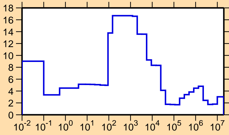
\Delta\sigma/\sigma vs. E for ^{70}\text{As}(n,\text{tot.})
