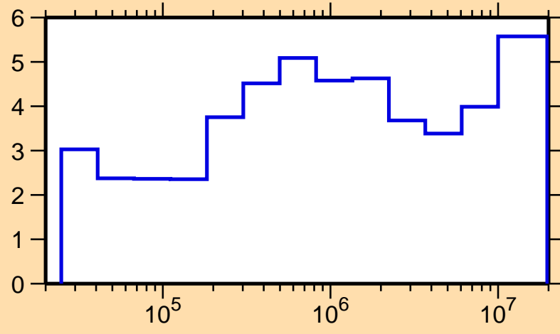
\Delta\sigma/\sigma vs. E for ^{70}\text{As}(n,\text{el.})
