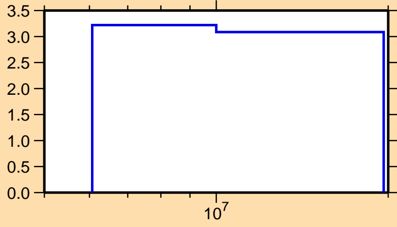
\Delta\sigma/\sigma vs. E for ^{70}\text{As}(n,\text{nonel.})
