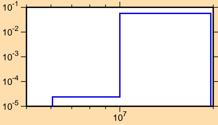
\sigma vs. E for ^{70}\text{As}(n,2n)
