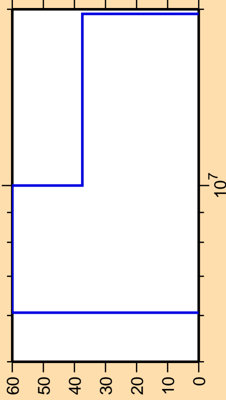
\Delta\sigma/\sigma vs. E for ^{70}\text{As}(n,2n)
