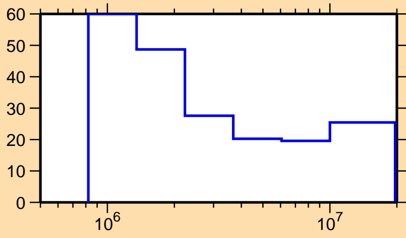
\Delta\sigma/\sigma vs. E for ^{70}\text{As}(n,n\text{cont.})
