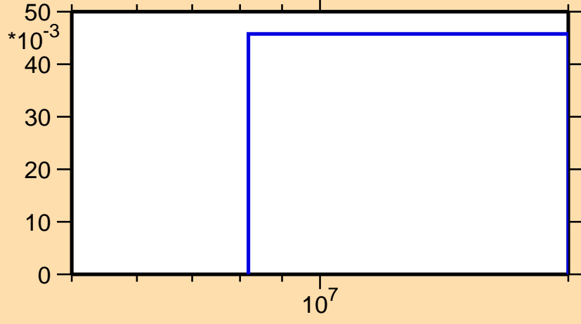
\sigma vs. E for ^{70}\text{As}(n,2n)
