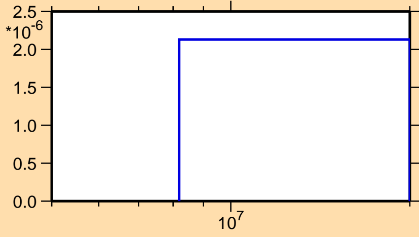
\sigma vs. E for ^{70}\text{As}(n,\text{pd})
