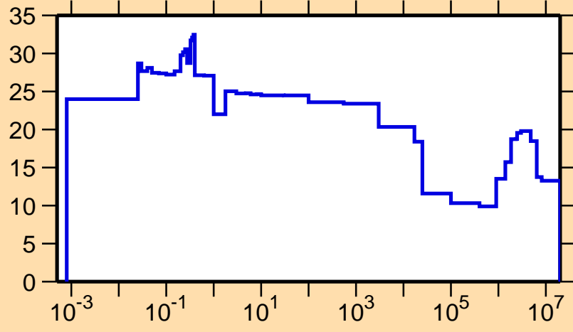
\Delta\sigma/\sigma vs. E for ^{70}\text{As}(n,p)
