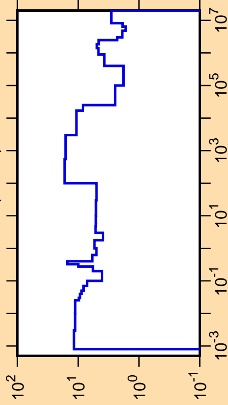
\Delta\sigma/\sigma vs. E for ^{70}\text{As}(n,\text{tot.})
