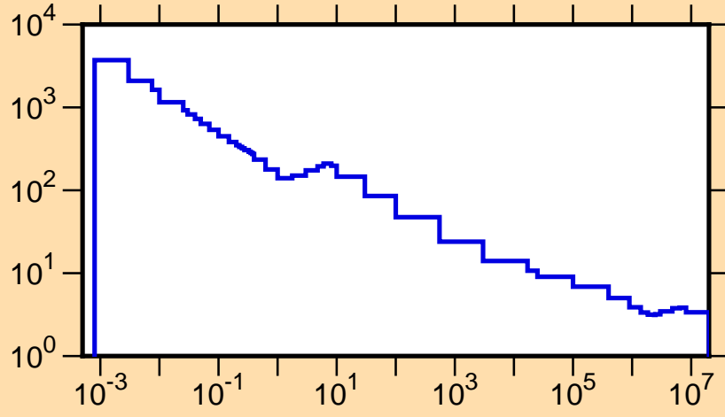
\sigma vs. E for ^{70}\text{As}(n,\text{tot.})
