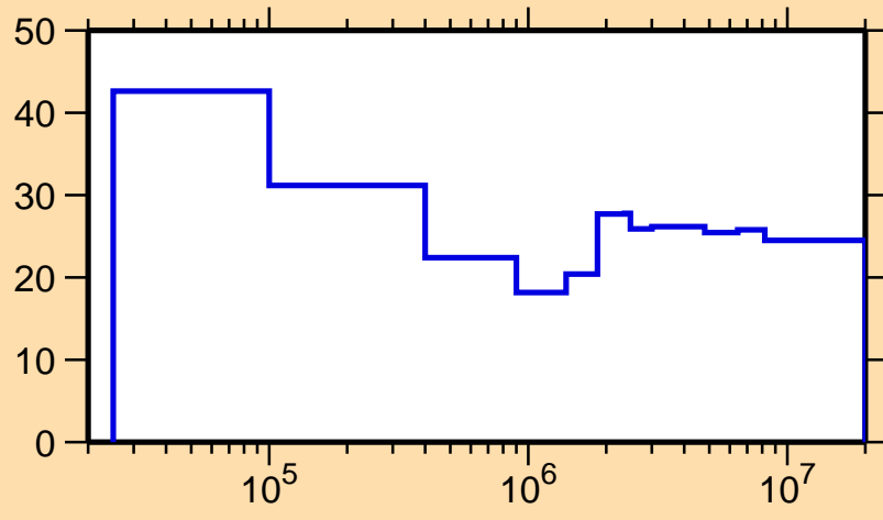
\Delta\sigma/\sigma vs. E for ^{70}\text{As}(n,n_1)
