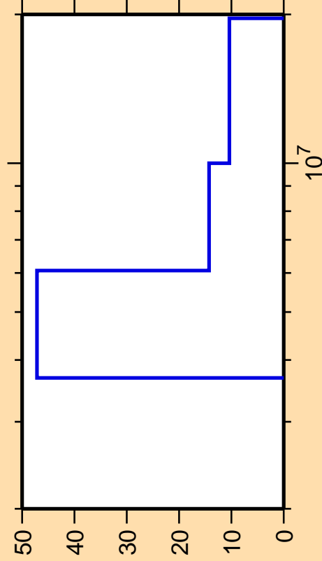
\Delta\sigma/\sigma vs. E for ^{71}\text{As}(n,np)
