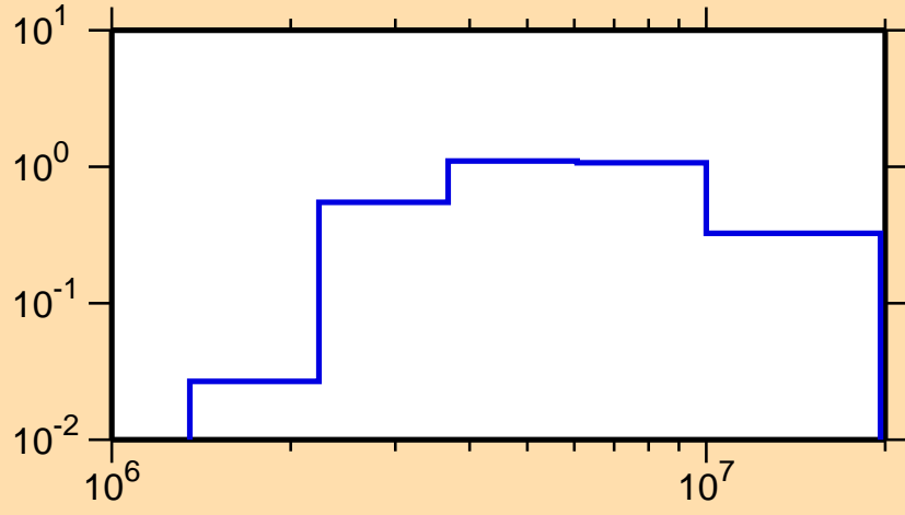
\sigma vs. E for ^{71}\text{As}(n,n\text{cont.})
