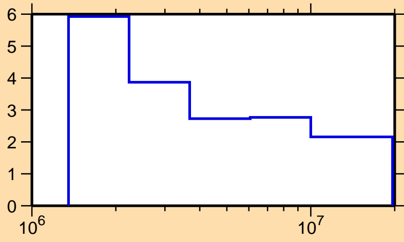
\Delta\sigma/\sigma vs. E for ^{71}\text{As}(n,n\text{onel.})
