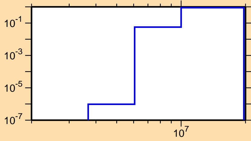
\sigma vs. E for ^{71}\text{As}(n,np)
