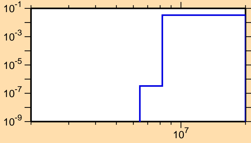
\sigma vs. E for ^{71}\text{As}(n,n\alpha)
