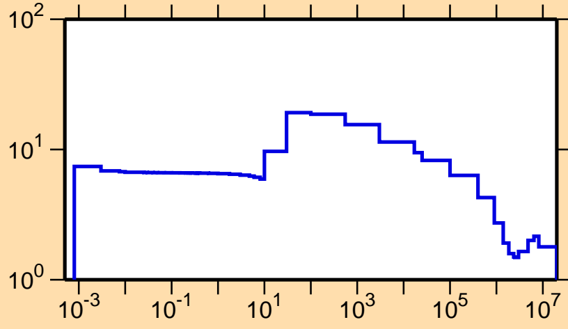
\sigma vs. E for ^{71}\text{As}(n,\text{el.})
