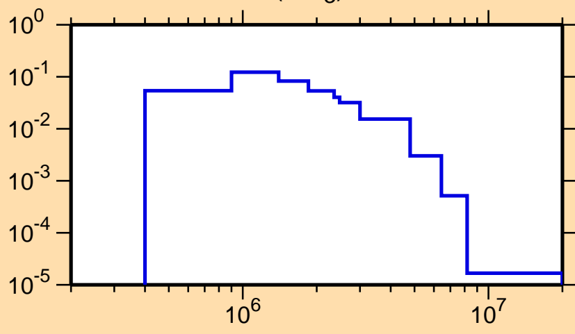
\sigma vs. E for ^{71}\text{As}(n,n_3)
