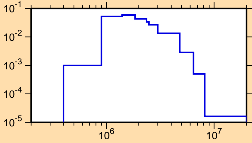
\sigma vs. E for ^{71}\text{As}(n,n_4)
