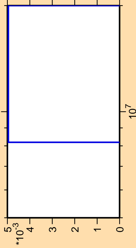
\Delta\sigma/\sigma vs. E for ^{71}\text{As} (mt 34)
