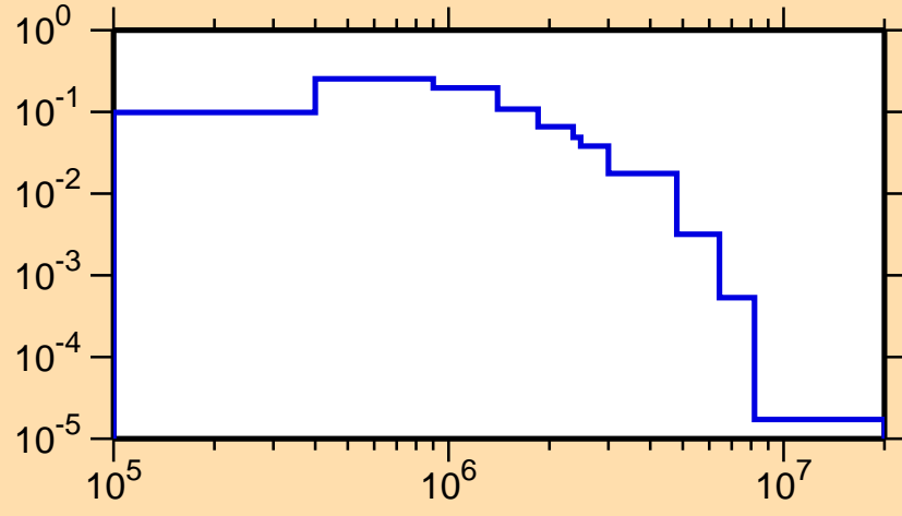
\sigma vs. E for ^{71}\text{As}(n,n_2)
