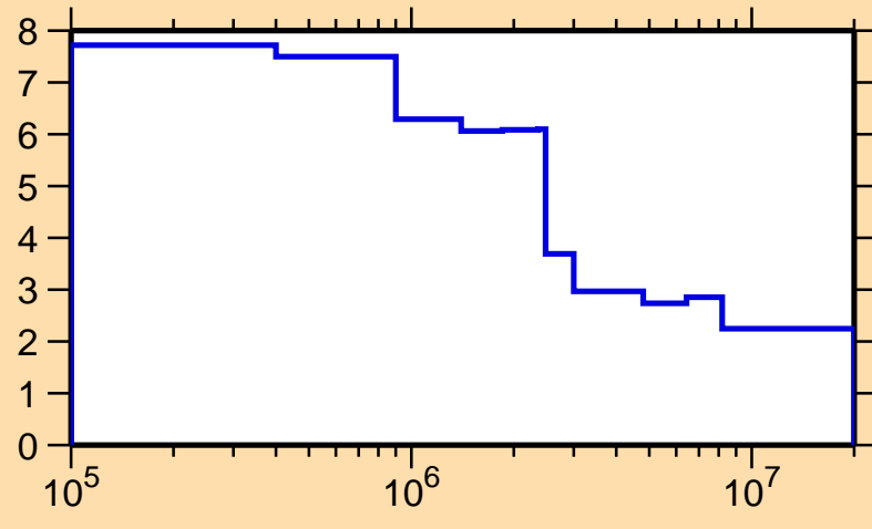
\Delta\sigma/\sigma vs. E for ^{71}\text{As}(n,\text{nonel.})
