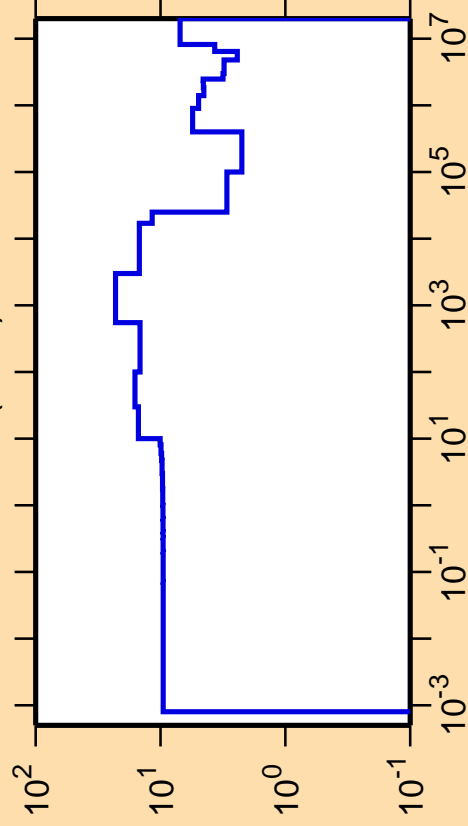
\Delta\sigma/\sigma vs. E for ^{71}\text{As}(n,\text{el.})
