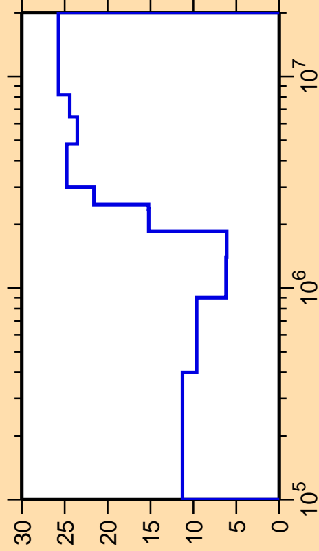
\Delta\sigma/\sigma vs. E for ^{71}\text{As}(n,n_2)
