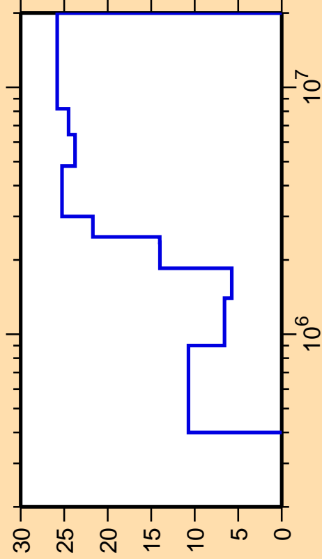
\Delta\sigma/\sigma vs. E for ^{71}\text{As}(n,n_3)
