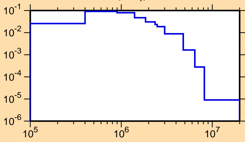
\sigma vs. E for ^{71}\text{As}(n,n_1)
