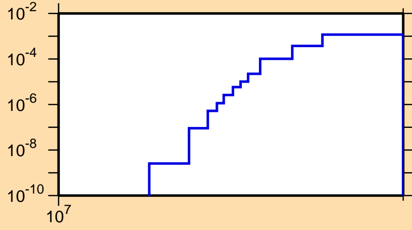
\sigma vs. E for ^{72}\text{As}(n,nd)
