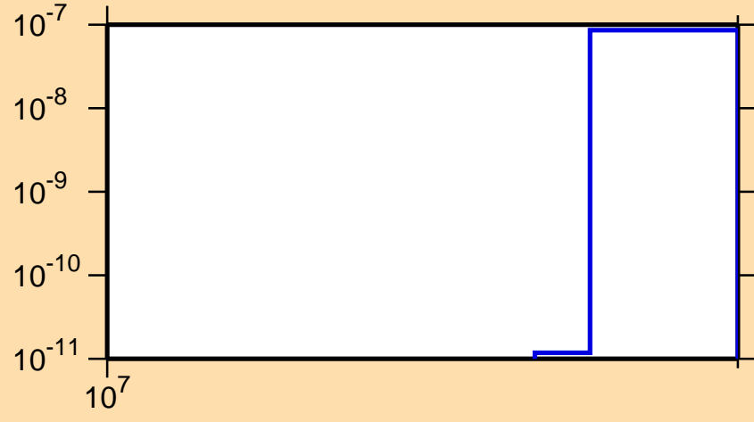
\sigma vs. E for ^{72}\text{As}(n,pt)
