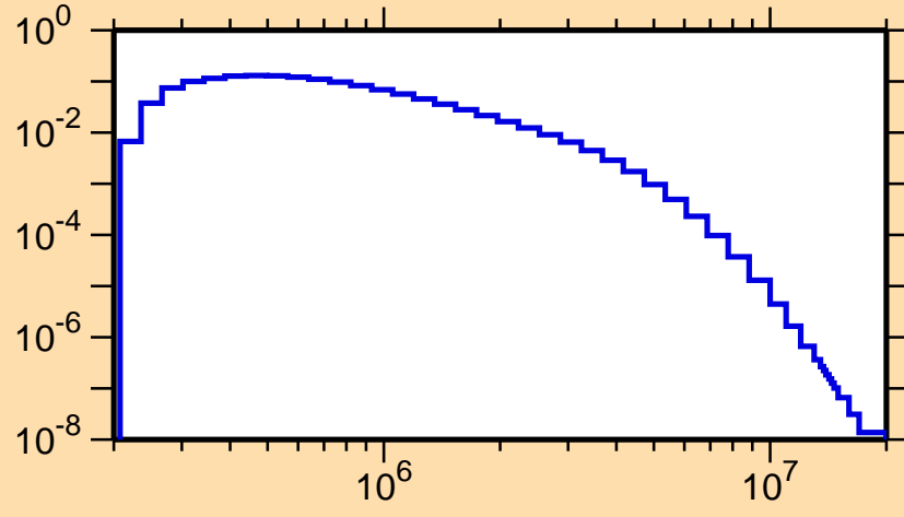
\sigma vs. E for ^{72}\text{As}(n,n_2)
