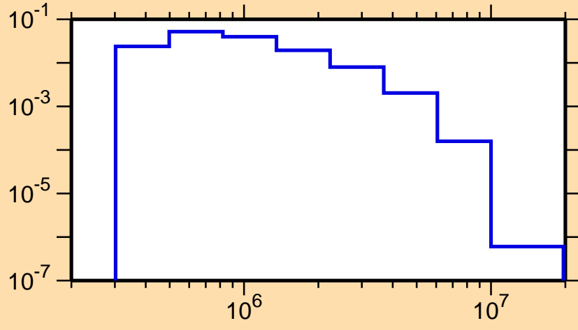
\sigma vs. E for ^{72}\text{As}(n,n_4)
