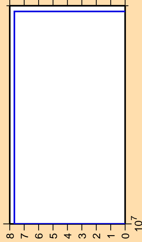
\Delta\sigma/\sigma vs. E for ^{72}\text{As} (mt 34)
