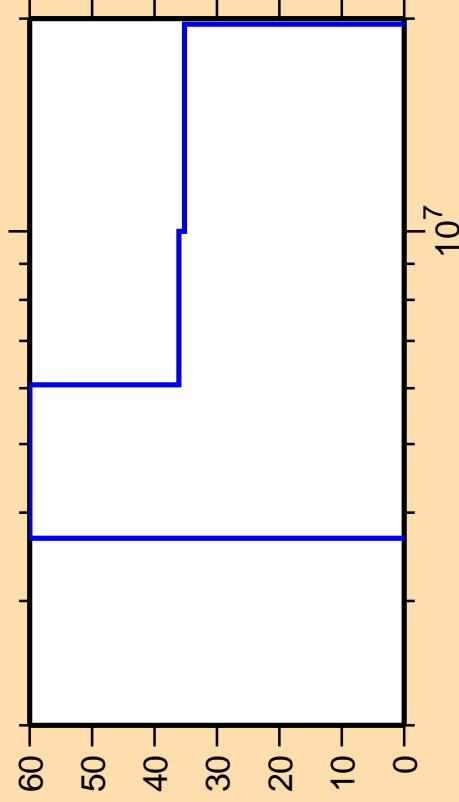
\Delta\sigma/\sigma vs. E for ^{72}\text{As}(n,p\alpha)
