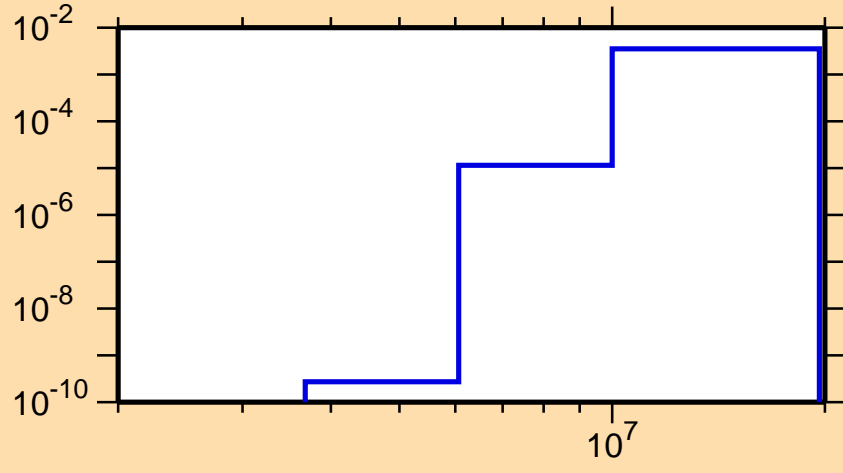
\sigma vs. E for ^{72}\text{As}(n,p\alpha)
