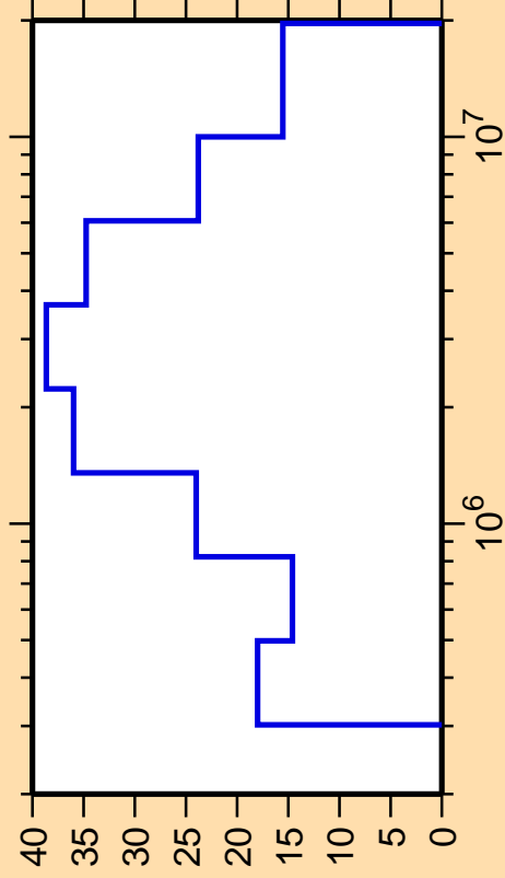
\Delta\sigma/\sigma vs. E for ^{72}\text{As}(n,n_4)
