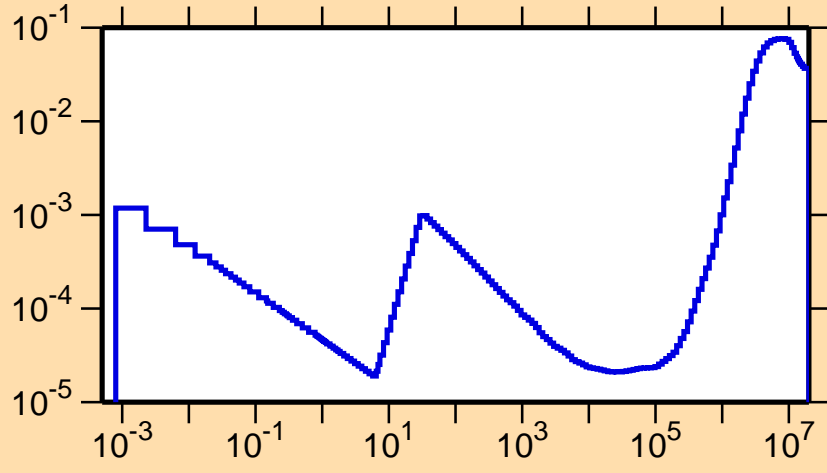
\sigma vs. E for ^{73}\text{As}(n,p)
