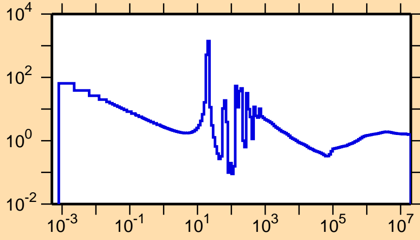
\sigma vs. E for ^{73}\text{As}(n,\text{nonel.})
