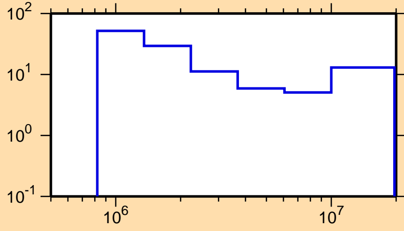
\Delta\sigma/\sigma vs. E for ^{73}\text{As}(n,n\text{cont.})
