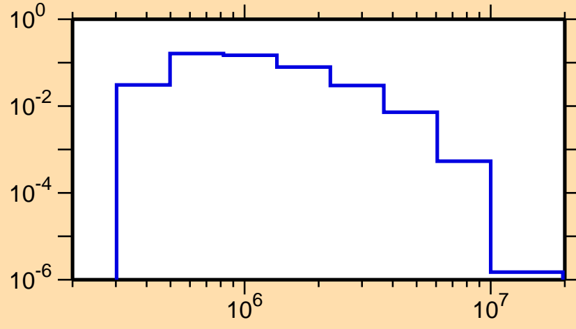
\sigma vs. E for ^{73}\text{As}(n,n_4)
