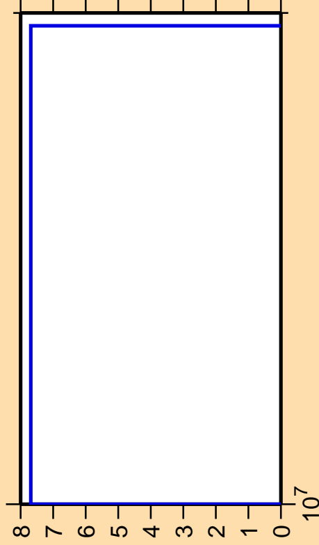
\Delta\sigma/\sigma vs. E for ^{73}\text{As}(n,pd)
