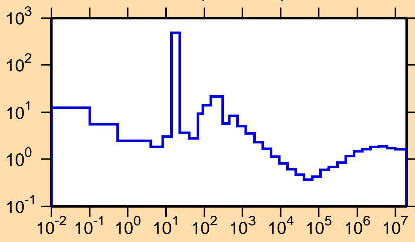
\sigma vs. E for ^{73}\text{As}(n,\text{nonel.})
