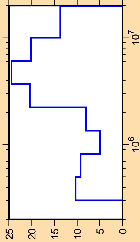
\Delta\sigma/\sigma vs. E for ^{73}\text{As}(n,n_4)
