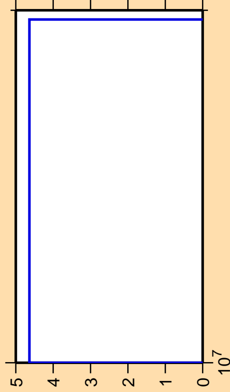
\Delta\sigma/\sigma vs. E for ^{73}\text{As}(n,2n\alpha)
