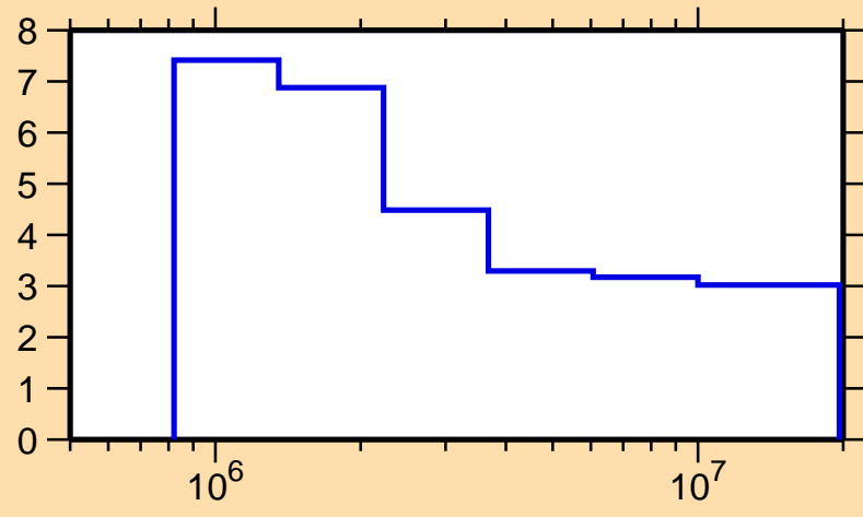
\Delta\sigma/\sigma vs. E for ^{73}\text{As}(n,n\text{onel.})
