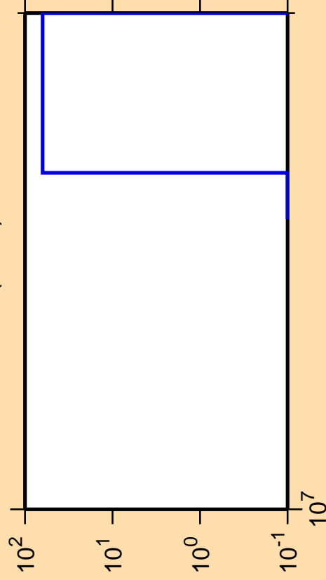
\Delta\sigma/\sigma vs. E for ^{75}\text{As}(n,nd)
