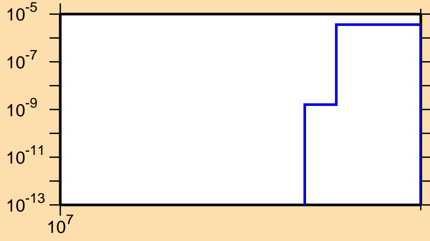
\sigma vs. E for ^{75}\text{As}(n,nd)
