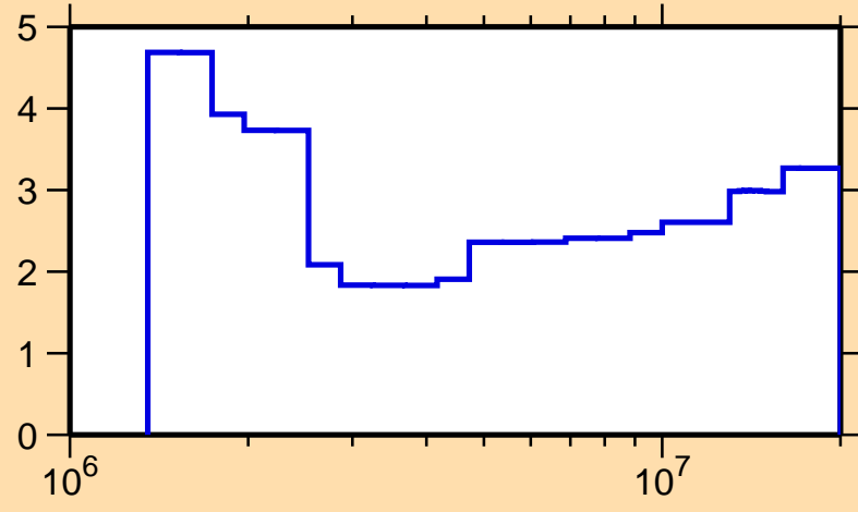
\Delta\sigma/\sigma vs. E for ^{75}\text{As}(n,n\text{oncl.})
