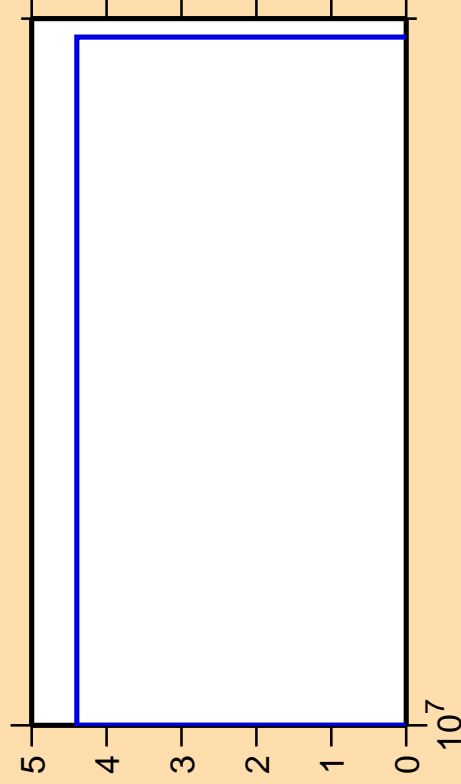
\Delta\sigma/\sigma vs. E for ^{75}\text{As}(n,2n)
