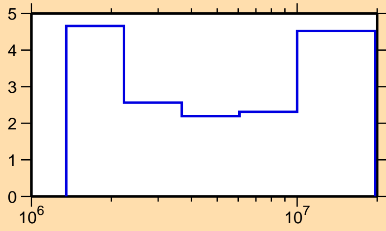
\Delta\sigma/\sigma vs. E for ^{75}\text{As}(n,n\text{cont.})
