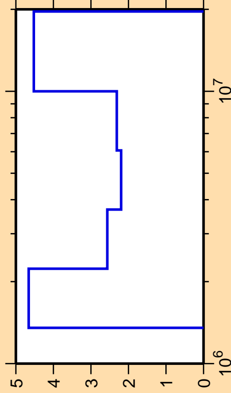
\Delta\sigma/\sigma vs. E for ^{75}\text{As}(n,n\text{cont.})
