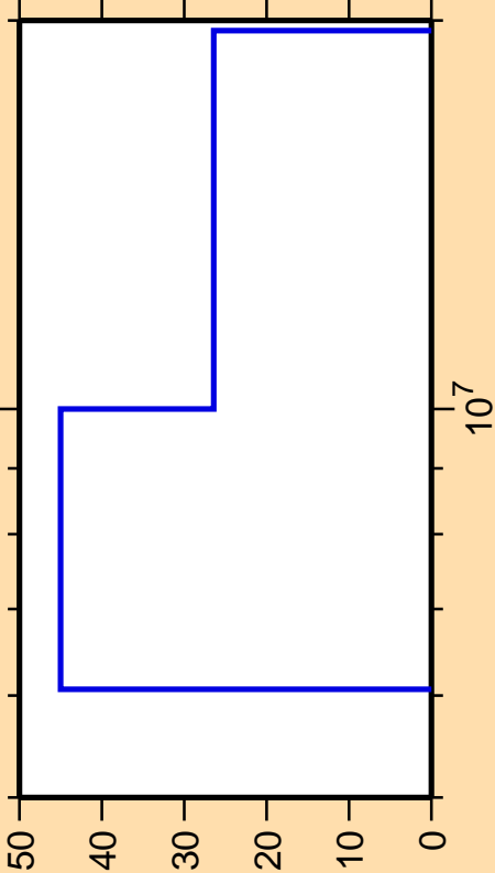
\Delta\sigma/\sigma vs. E for ^{75}\text{As}(n,n\alpha)
