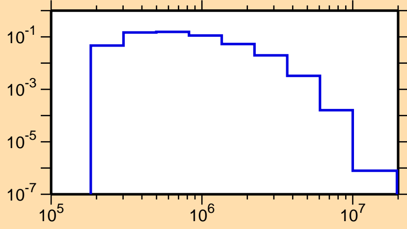
\sigma vs. E for ^{75}\text{As}(n,n_1)
