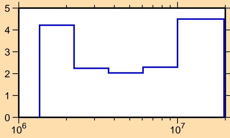
\Delta\sigma/\sigma vs. E for ^{75}\text{As}(n,\text{inel.})
