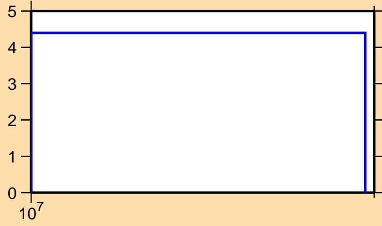
\Delta\sigma/\sigma vs. E for ^{75}\text{As}(n,2n)
