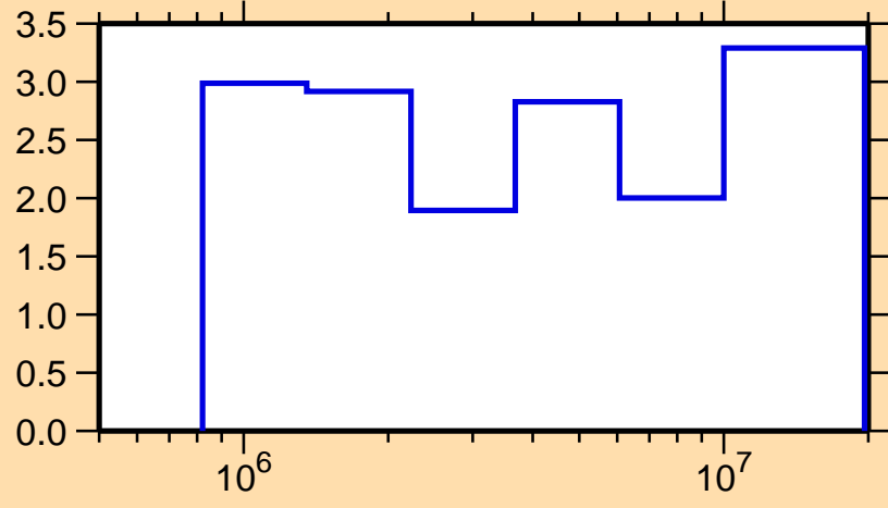
\Delta\sigma/\sigma vs. E for ^{75}\text{As}(n,el.)
