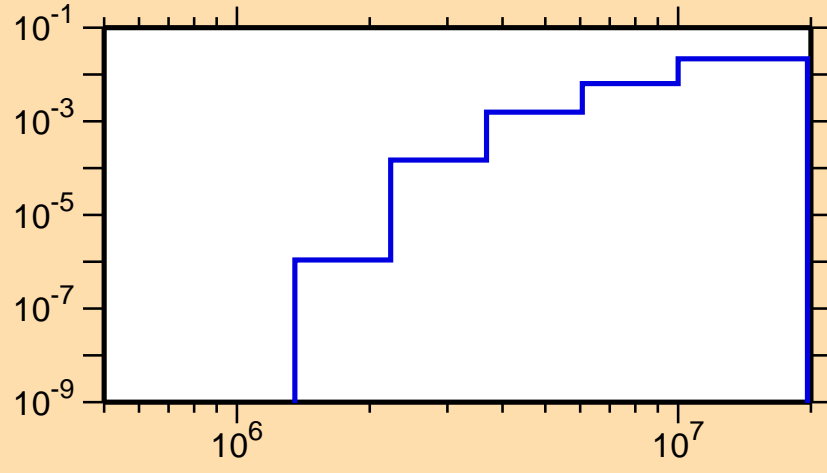
\sigma vs. E for ^{75}\text{As}(n,p)
