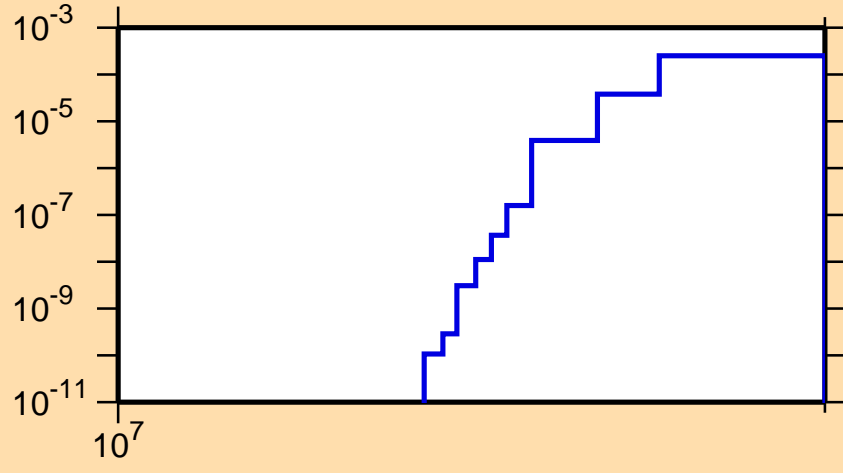
\sigma vs. E for ^{76}\text{As}(n,nd)
