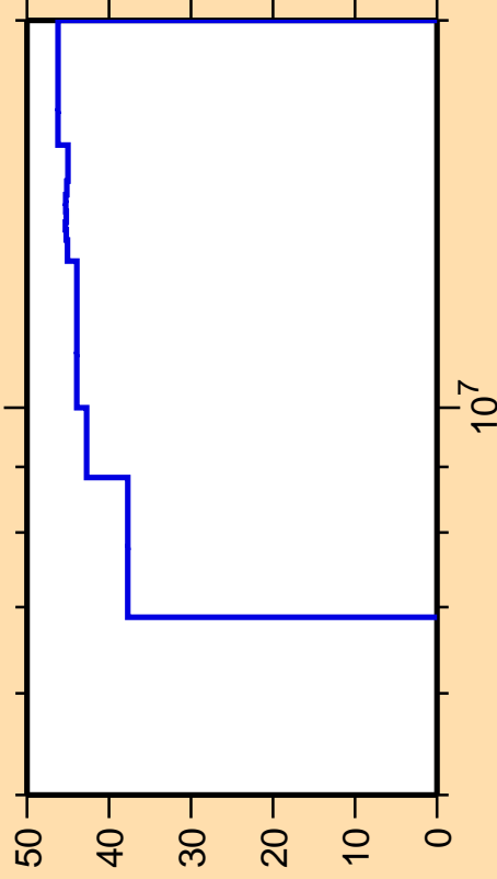
\Delta\sigma/\sigma vs. E for ^{78}\text{As}(n,\gamma)
