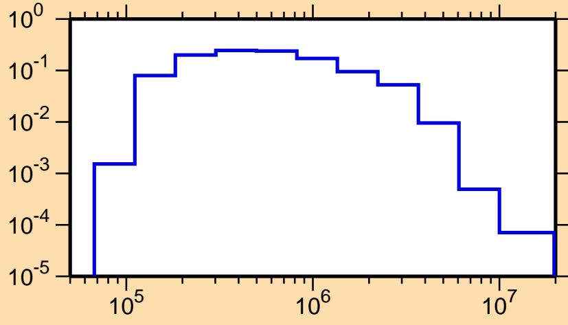
\sigma vs. E for ^{79}\text{As}(n,n_1)
