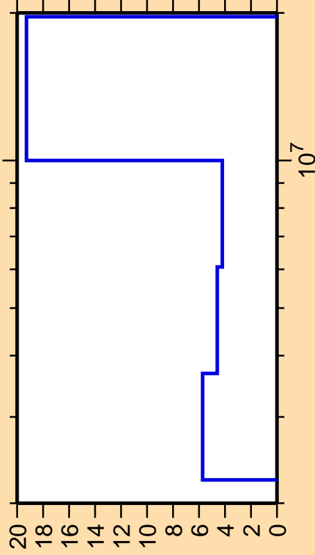
\Delta\sigma/\sigma vs. E for ^{79}\text{As}(n,n\text{cont.})
