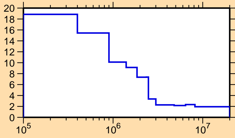
\Delta\sigma/\sigma vs. E for ^{79}\text{As}(n,\text{nonel.})
