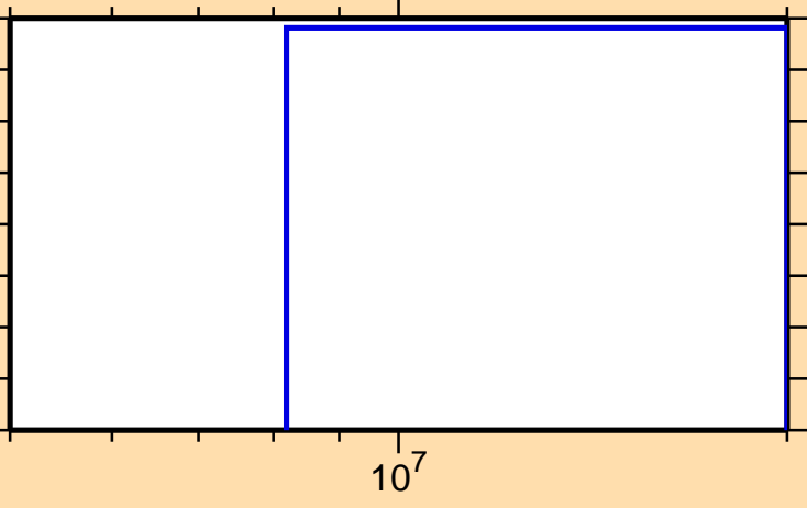
\sigma vs. E for ^{79}\text{As}(n,\text{nd})
