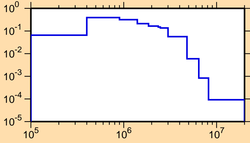
\sigma vs. E for ^{79}\text{As}(n,n_3)
