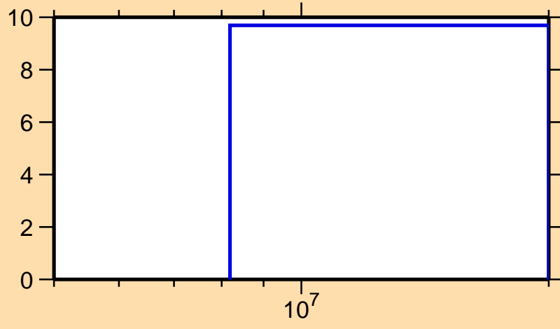
\Delta\sigma/\sigma vs. E for ^{79}\text{As}(n,\text{inel.})
