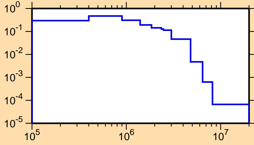
\sigma vs. E for ^{79}\text{As}(n,n_2)
