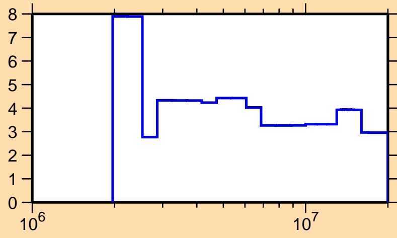
\Delta\sigma/\sigma vs. E for ^{80}\text{As}(n,n\text{oncl.})
