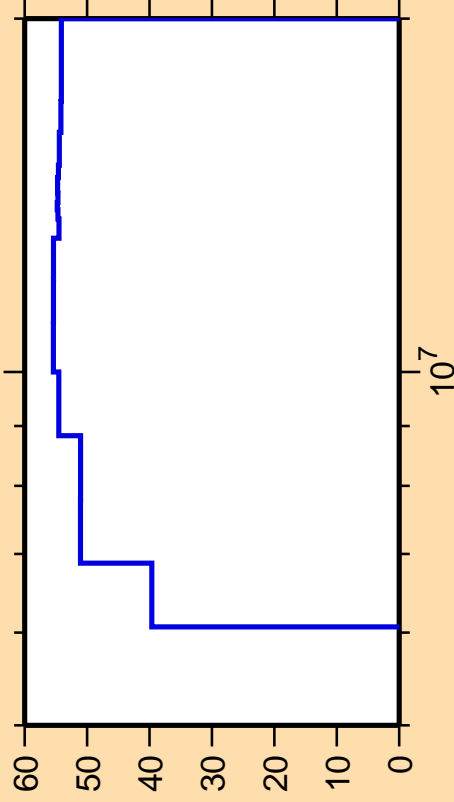
\Delta\sigma/\sigma vs. E for ^{80}\text{As}(n,\gamma)
