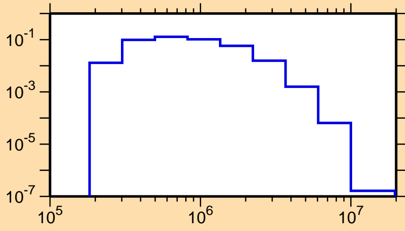
\sigma vs. E for ^{80}\text{As}(n,n_1)
