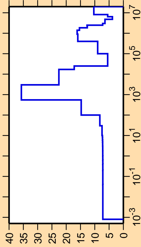
\Delta\sigma/\sigma vs. E for ^{80}\text{As}(n,\text{el.})
