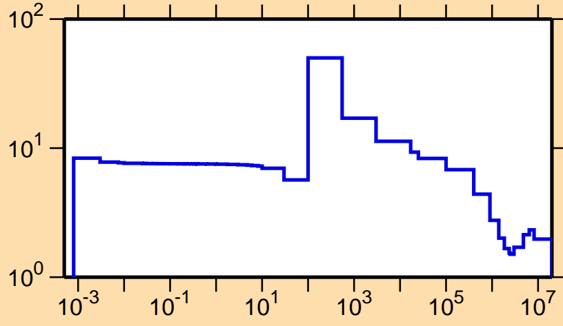
\sigma vs. E for ^{80}\text{As}(n,\text{el.})
