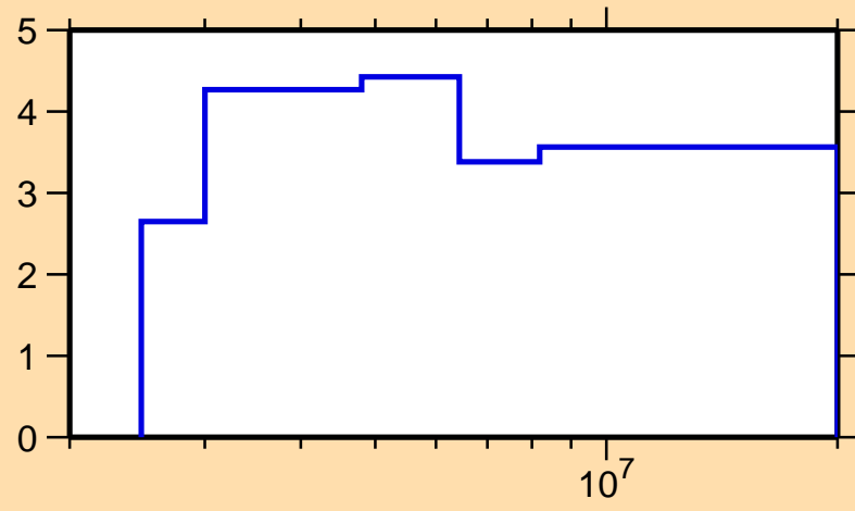
\Delta\sigma/\sigma vs. E for ^{80}\text{As}(n,\text{nonel.})
