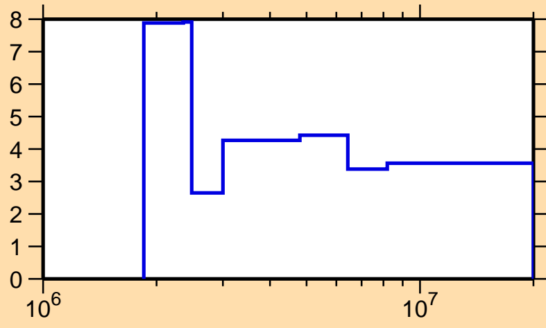
\Delta\sigma/\sigma vs. E for ^{80}\text{As}(n,n\text{onel.})
