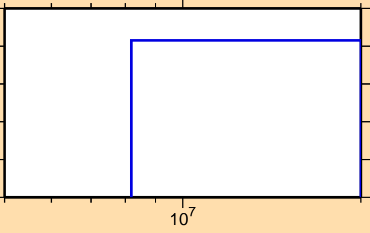
\sigma vs. E for ^{80}\text{As}(n,n\alpha)
