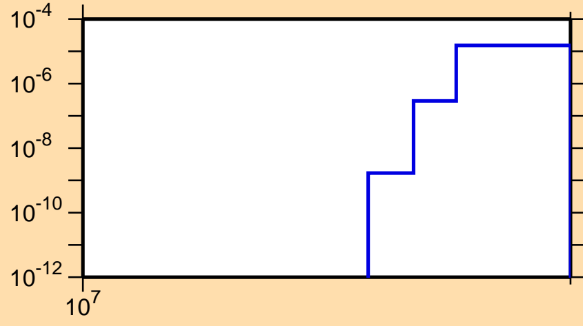
\sigma vs. E for ^{82}\text{As}(n,\text{nd})
