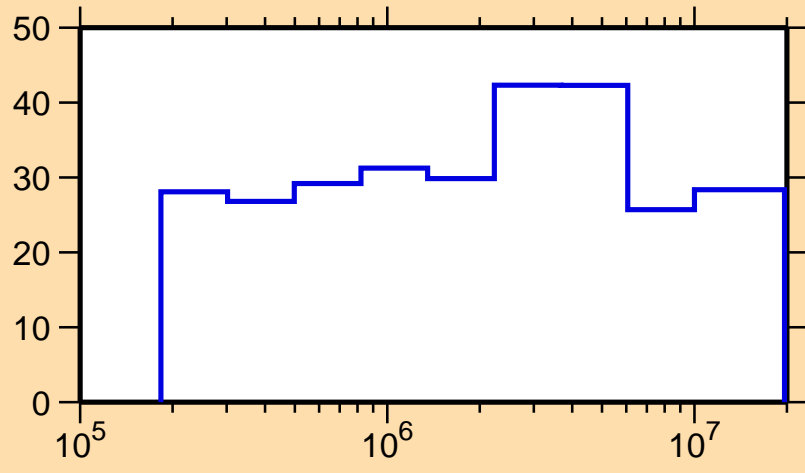
\Delta\sigma/\sigma vs. E for ^{82}\text{As}(n,n_1)
