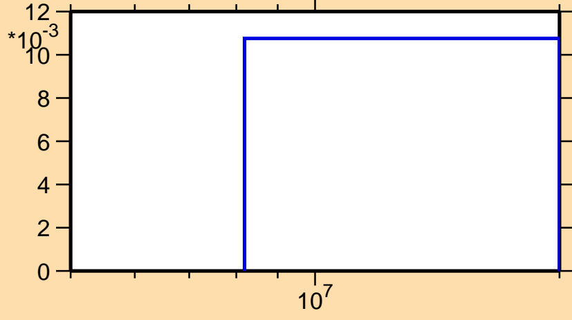
\sigma vs. E for ^{82}\text{As}(n,3n)
