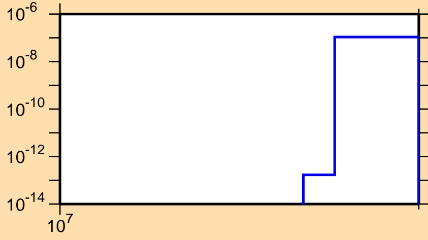
\sigma vs. E for ^{82}\text{As}(n,2np)
