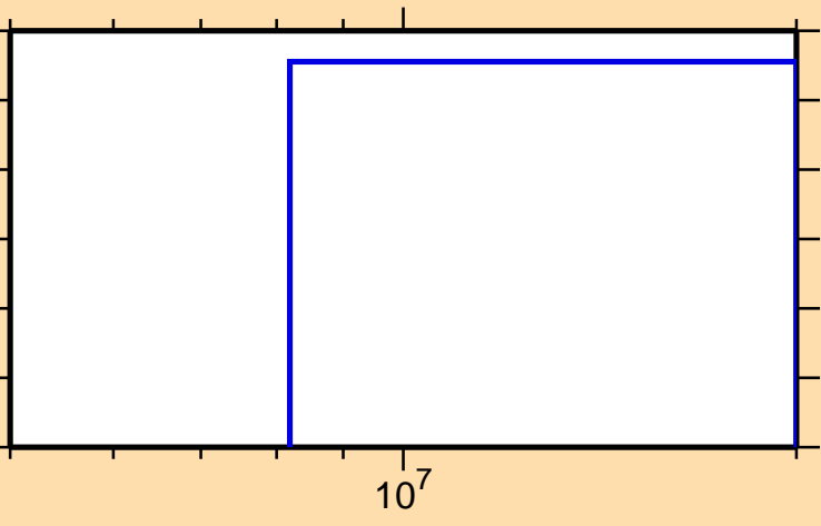
\sigma vs. E for ^{82}\text{As}(n,3n)
