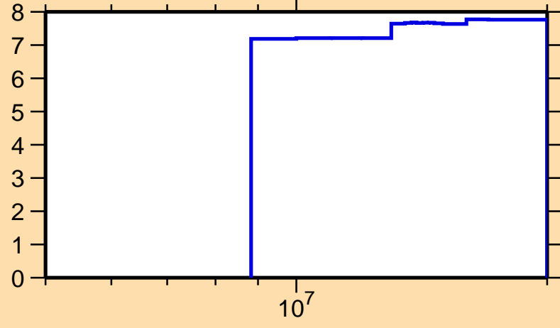
\Delta\sigma/\sigma vs. E for ^{83}\text{As}(n,\text{nonel.})
