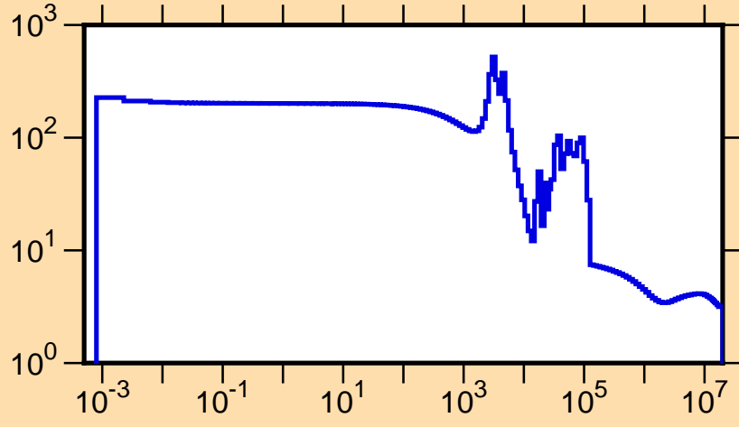
\sigma vs. E for ^{83}\text{As}(n,\text{tot.})
