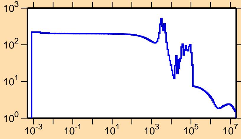
\sigma vs. E for ^{83}\text{As}(n,\text{el.})
