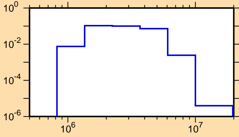
\sigma vs. E for ^{83}\text{As}(n,n_3)
