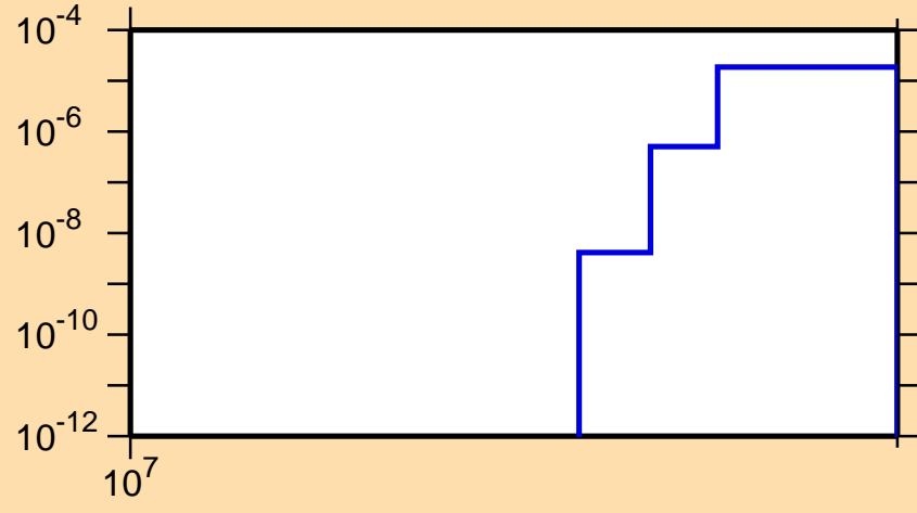
\sigma vs. E for ^{84}\text{As}(n,\text{nd})
