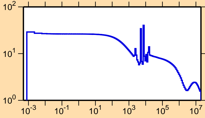
\sigma vs. E for ^{84}\text{As}(n,\text{el.})
