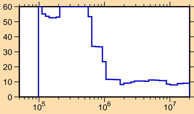
\Delta\sigma/\sigma vs. E for ^{84}\text{As}(n,\text{nonel.})
