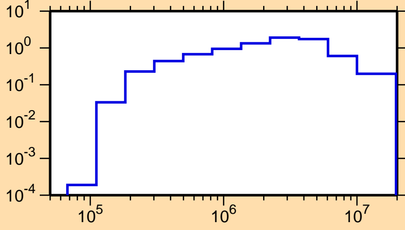
\sigma vs. E for ^{84}\text{As}(n,\text{inel.})
