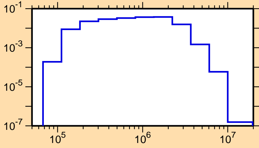
\sigma vs. E for ^{84}\text{As}(n,n_1)
