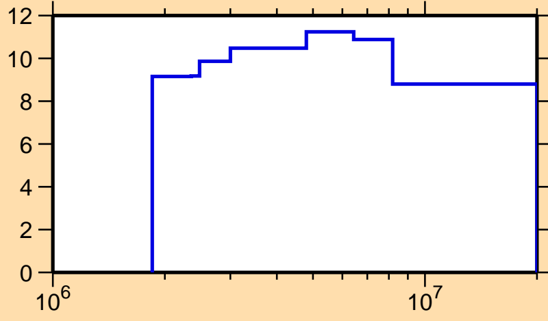
\Delta\sigma/\sigma vs. E for ^{84}\text{As}(n,n\text{onel.})
