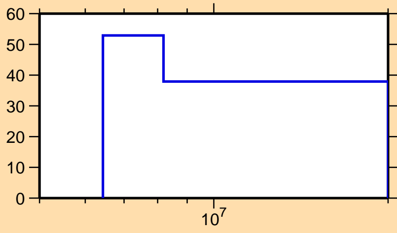
\Delta\sigma/\sigma vs. E for ^{84}\text{As}(n,p)
