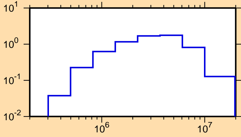
\sigma vs. E for ^{85}\text{As}(n,n\text{cont.})
