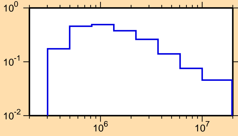
\sigma vs. E for ^{85}\text{As}(n,n_1)
