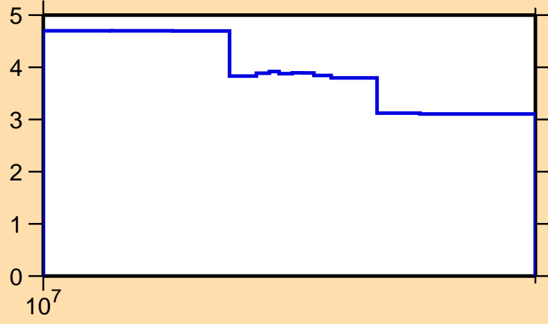
\Delta\sigma/\sigma vs. E for ^{197}\text{At}(n,\text{tot.})
