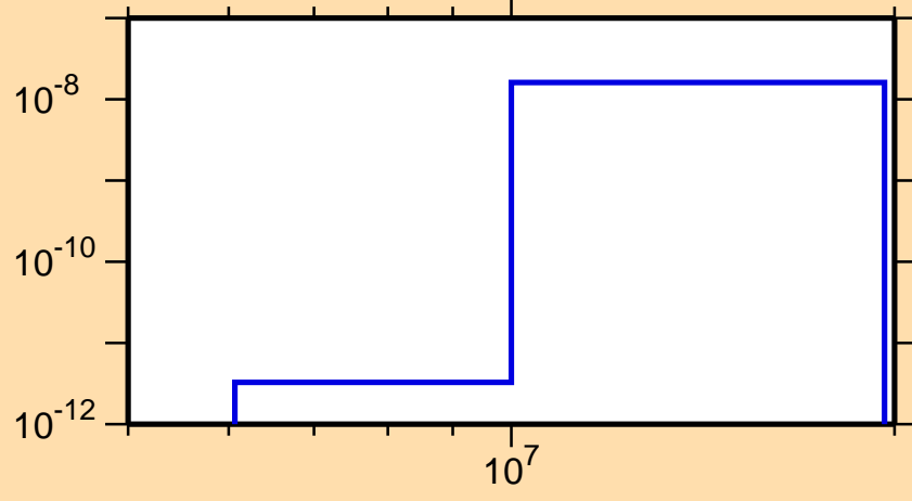
\sigma vs. E for ^{197}\text{At}(\text{mt117})
