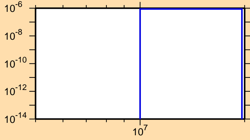
\sigma vs. E for ^{197}\text{At}(n,2n\alpha)
