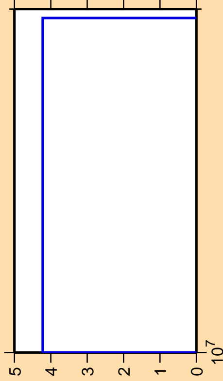
\Delta\sigma/\sigma vs. E for ^{197}\text{At}(n,3n)
