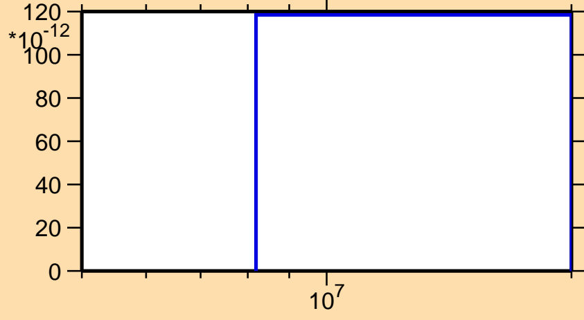
\sigma vs. E for ^{197}\text{At}(n,\text{pt})
