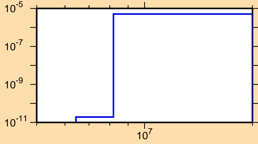
\sigma vs. E for ^{197}\text{At}(n,\text{He3})
