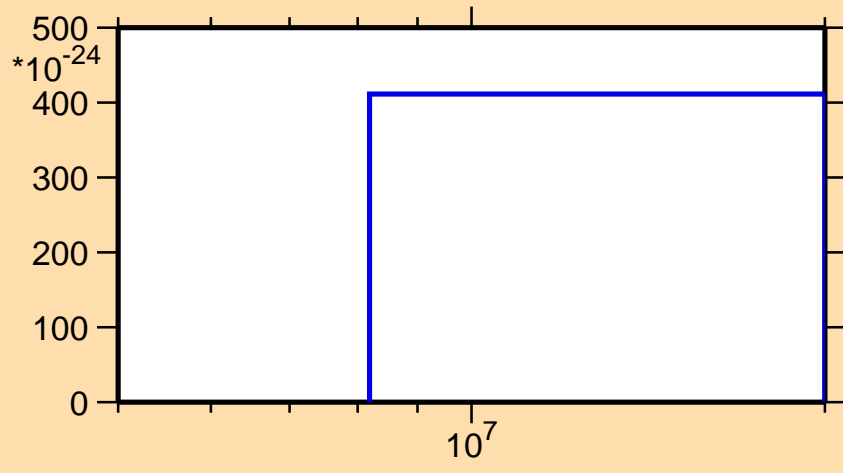
\sigma vs. E for ^{197}\text{At}(\text{mt } 42)
