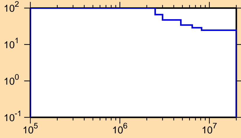
\Delta\sigma/\sigma vs. E for ^{197}\text{At}(n,n\text{cont.})
