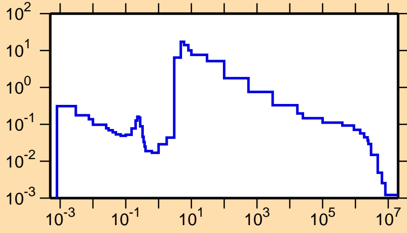
\sigma vs. E for ^{197}\text{At}(n,\gamma)
