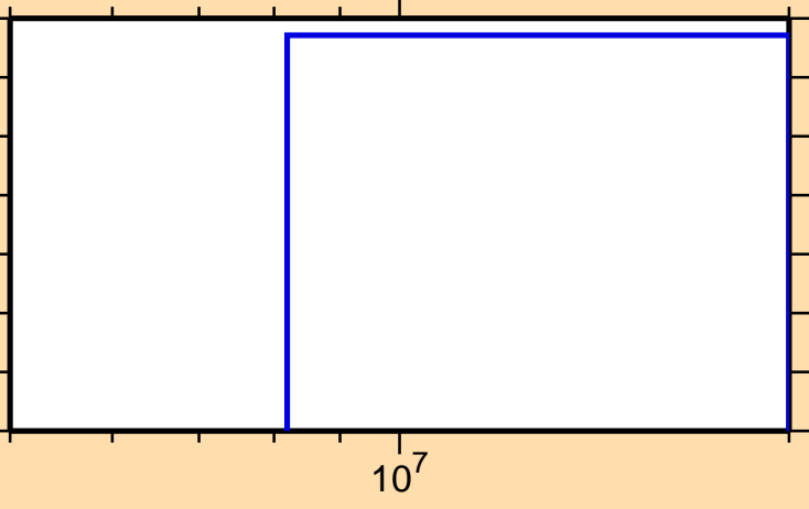
\sigma vs. E for ^{197}\text{At}(n,\text{nd})
