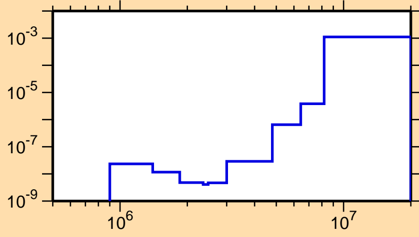
\sigma vs. E for ^{197}\text{At}(n,n\alpha)
