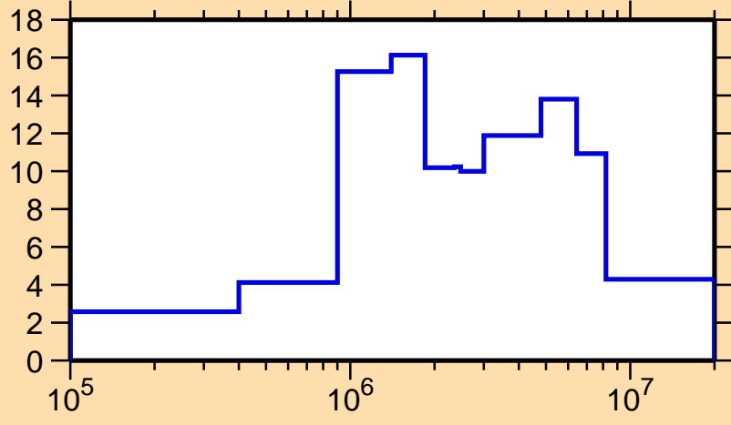
\Delta\sigma/\sigma vs. E for ^{197}\text{At}(n, el.)
