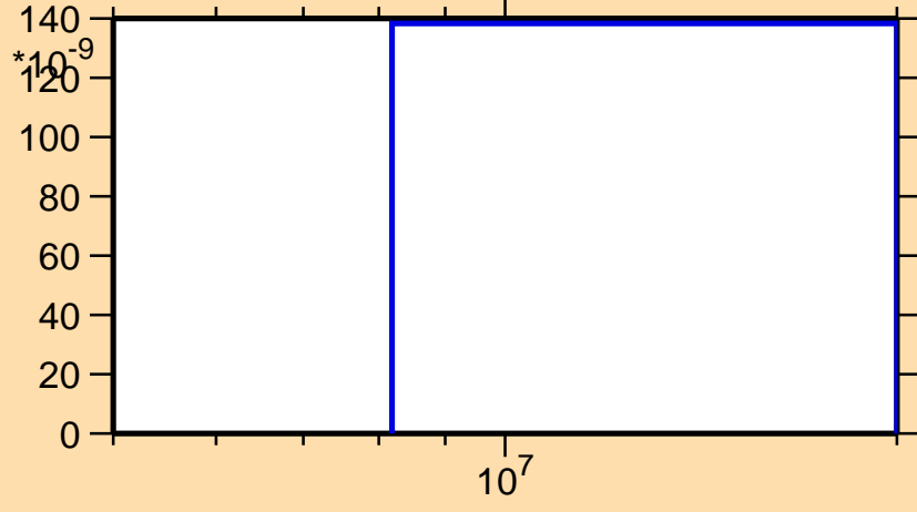
\sigma vs. E for ^{197}\text{At}(n,2np)
