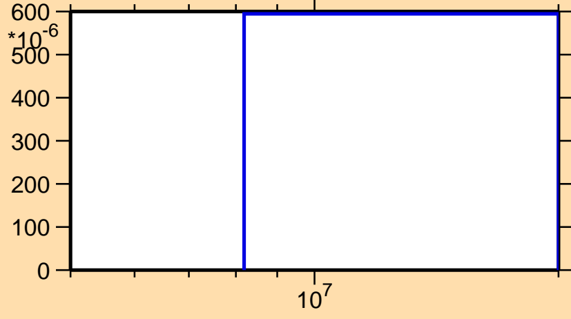
\sigma vs. E for ^{197}\text{At}(n,2n)
