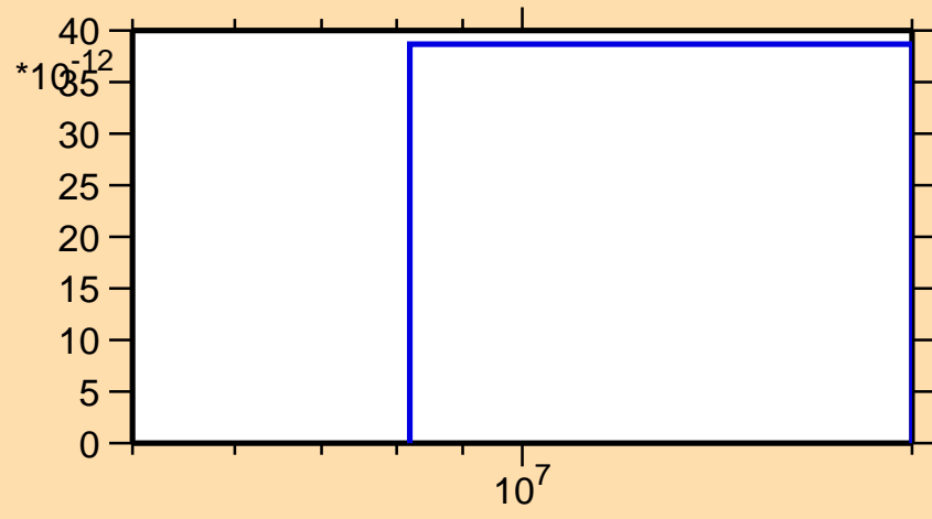
\sigma vs. E for ^{197}\text{At}(n,3n\alpha)
