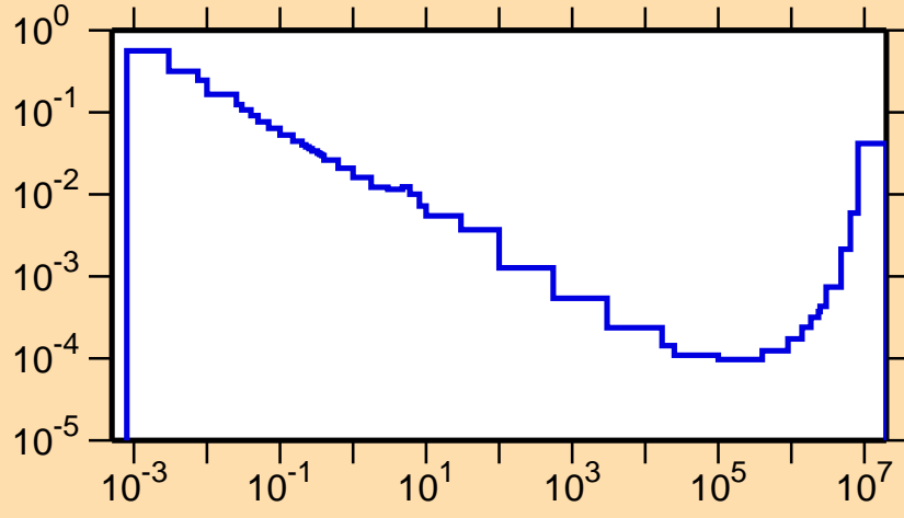
\sigma vs. E for ^{197}\text{At}(n,\alpha)
