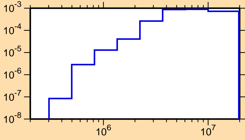
\sigma vs. E for ^{198}\text{At}(n,n_3)
