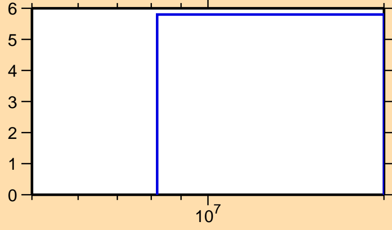
\Delta\sigma/\sigma vs. E for ^{198}\text{At}(n,\text{el.})
