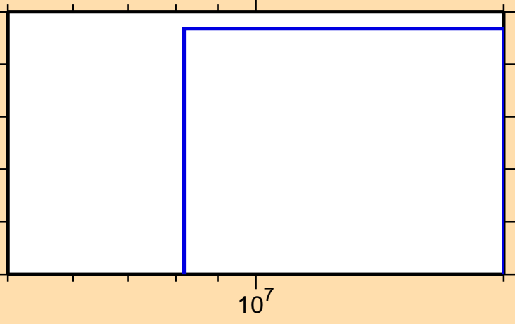
\sigma vs. E for ^{198}\text{At}(n,2n\alpha)
