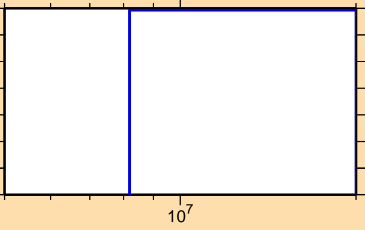
\sigma vs. E for ^{198}\text{At}(n,3n)
