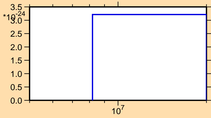
\sigma vs. E for ^{198}\text{At}(\text{mt } 42)
